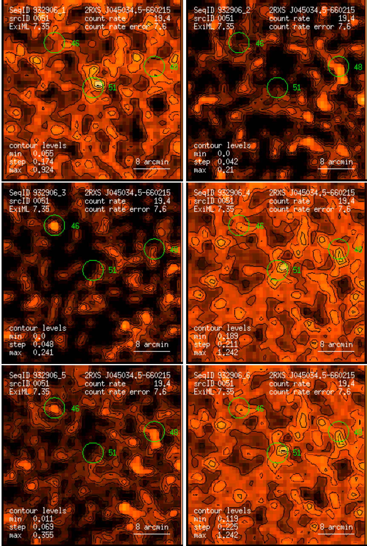
Figure 51: RASS 932906: detection 0051: band rate images, Gaussian filter: (1) PSPC channels 11 – 41, (2) 52 – 90, (3) 91 – 201, (4) 11 – 235, (5) 52 – 201, (6) 11 – 201. Broad band rates in counts/ks. Band rate contour levels in counts/ks/arcmin 2 .
