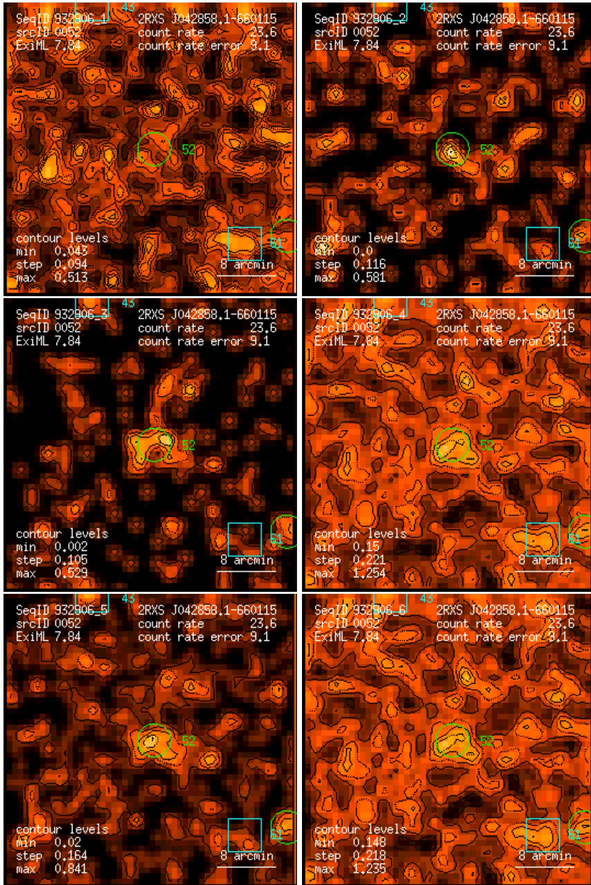
Figure 52: RASS 932906: detection 0052: band rate images, Gaussian filter: (1) PSPC channels 11 – 41, (2) 52 – 90, (3) 91 – 201, (4) 11 – 235, (5) 52 – 201, (6) 11 – 201. Broad band rates in counts/ks. Band rate contour levels in counts/ks/arcmin 2 .
