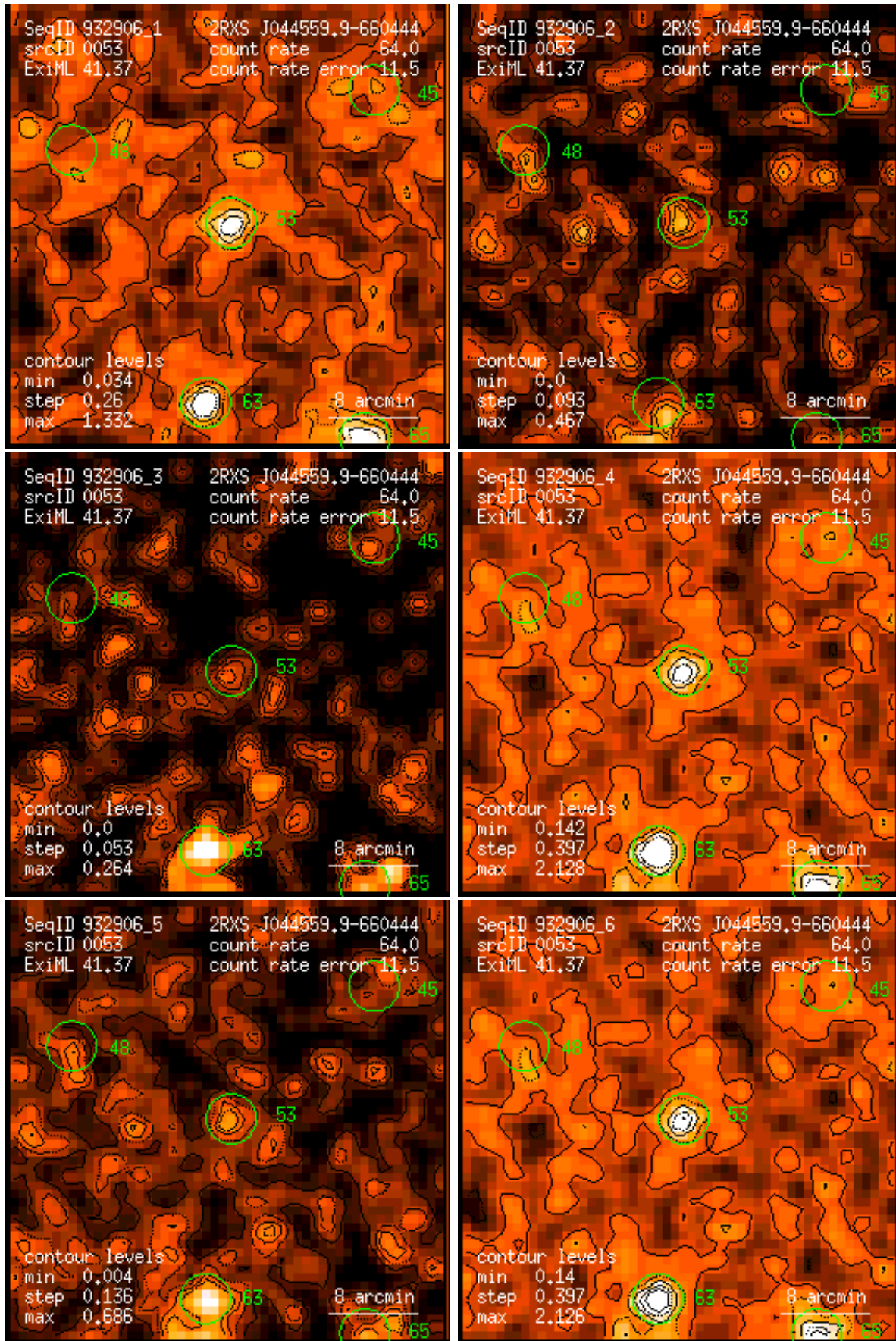
Figure 53: RASS 932906: detection 0053: band rate images, Gaussian filter: (1) PSPC channels 11 – 41, (2) 52 – 90, (3) 91 – 201, (4) 11 – 235, (5) 52 – 201, (6) 11 – 201. Broad band rates in counts/ks. Band rate contour levels in counts/ks/arcmin 2 .
