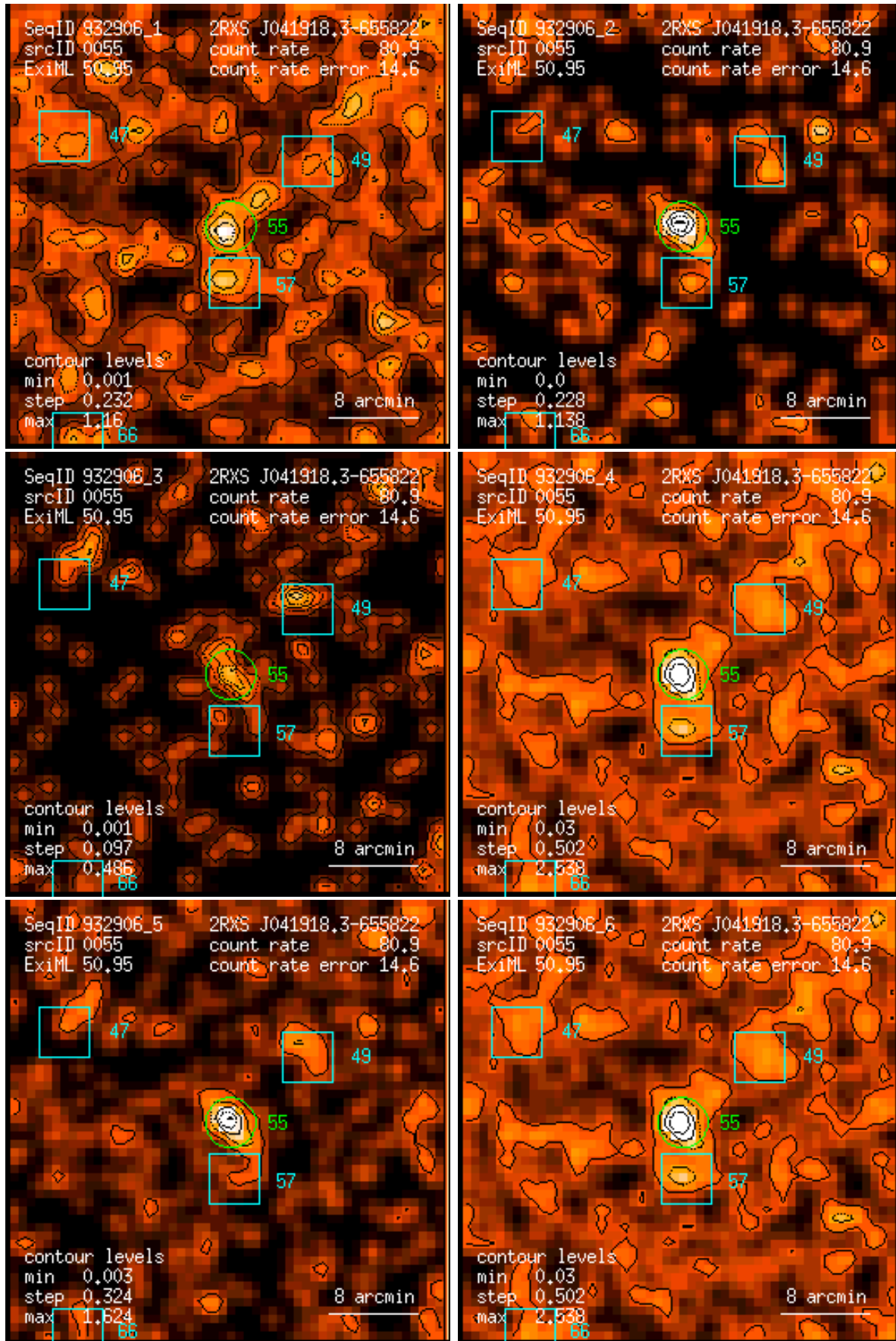
Figure 55: RASS 932906: detection 0055: band rate images, Gaussian filter: (1) PSPC channels 11 – 41, (2) 52 – 90, (3) 91 – 201, (4) 11 – 235, (5) 52 – 201, (6) 11 – 201. Broad band rates in counts/ks. Band rate contour levels in counts/ks/arcmin 2 .
