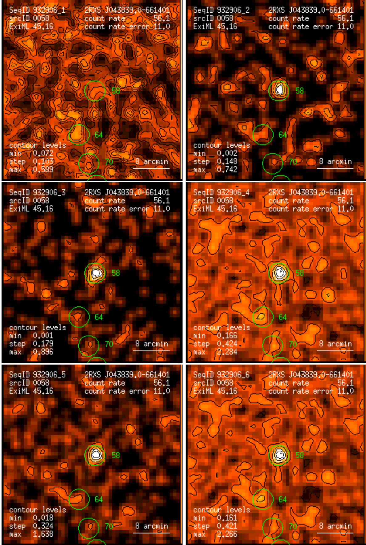
Figure 58: RASS 932906: detection 0058: band rate images, Gaussian filter: (1) PSPC channels 11 – 41, (2) 52 – 90, (3) 91 – 201, (4) 11 – 235, (5) 52 – 201, (6) 11 – 201. Broad band rates in counts/ks. Band rate contour levels in counts/ks/arcmin 2 .
