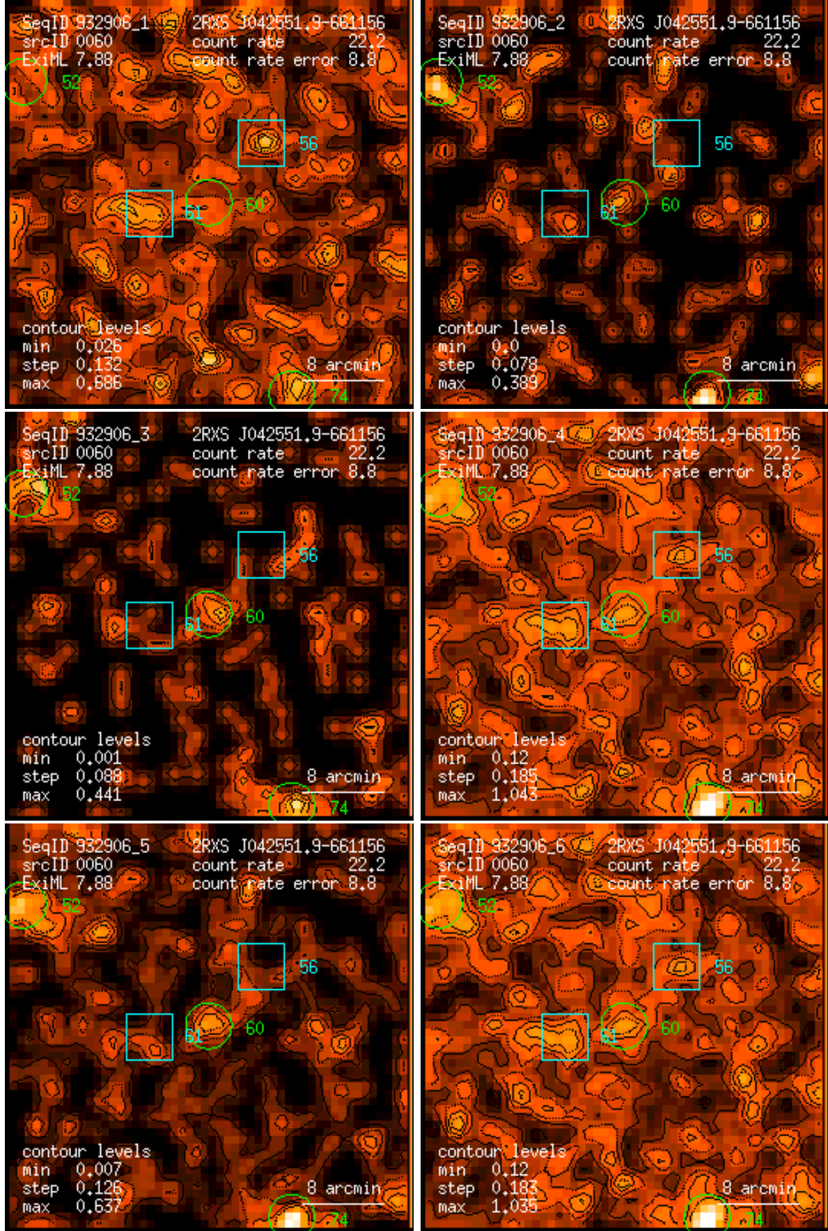
Figure 60: RASS 932906: detection 0060: band rate images, Gaussian filter: (1) PSPC channels 11 – 41, (2) 52 – 90, (3) 91 – 201, (4) 11 – 235, (5) 52 – 201, (6) 11 – 201. Broad band rates in counts/ks. Band rate contour levels in counts/ks/arcmin 2 .
