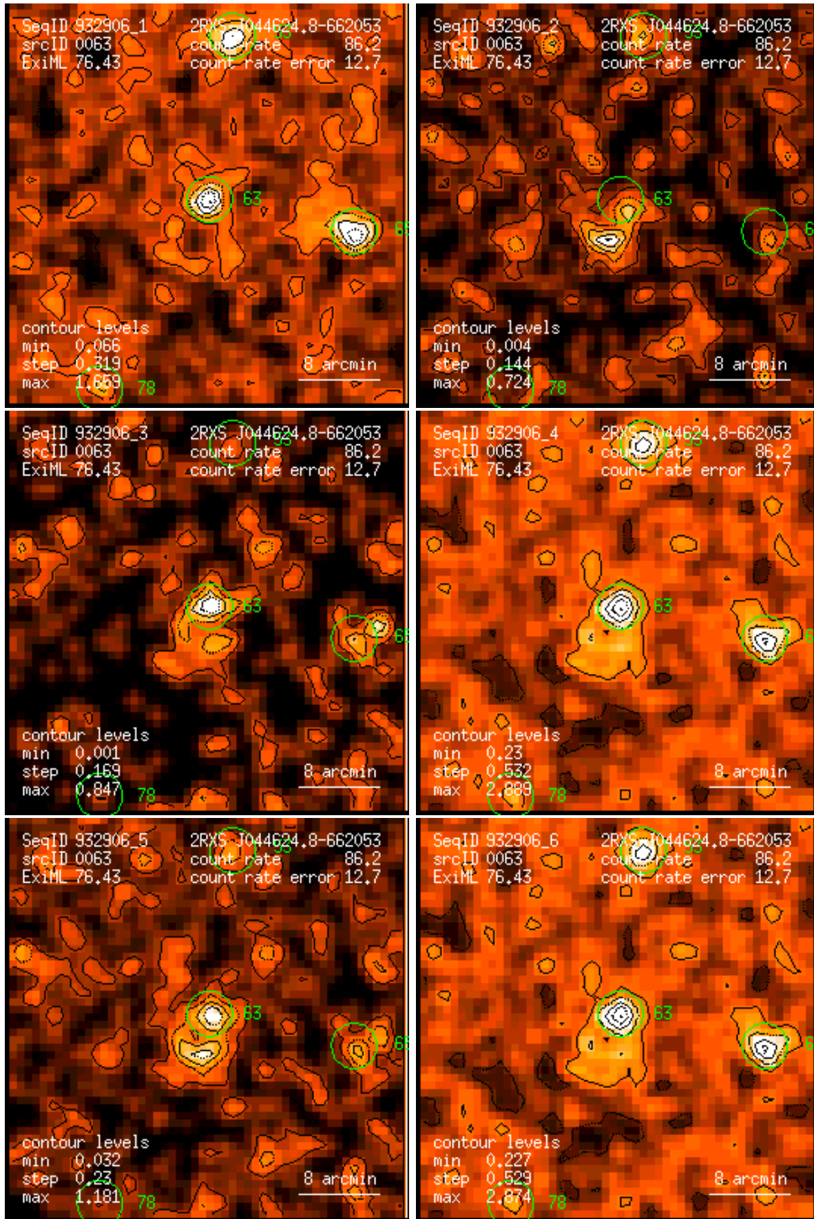
Figure 63: RASS 932906: detection 0063: band rate images, Gaussian filter: (1) PSPP channels 11 – 41, (2) 52 – 90, (3) 91 – 201, (4) 11 – 235, (5) 52 – 201, (6) 11 – 201. Broad band rates in counts/ks. Band rate contour levels in counts/ks/arcmin 2 .
