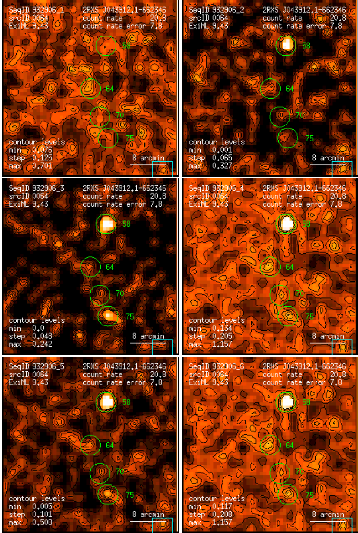
Figure 64: RASS 932906: detection 0064: band rate images, Gaussian filter: (1) PSPC channels 11 – 41, (2) 52 – 90, (3) 91 – 201, (4) 11 – 235, (5) 52 – 201, (6) 11 – 201. Broad band rates in counts/ks. Band rate contour levels in counts/ks/arcmin 2 .
