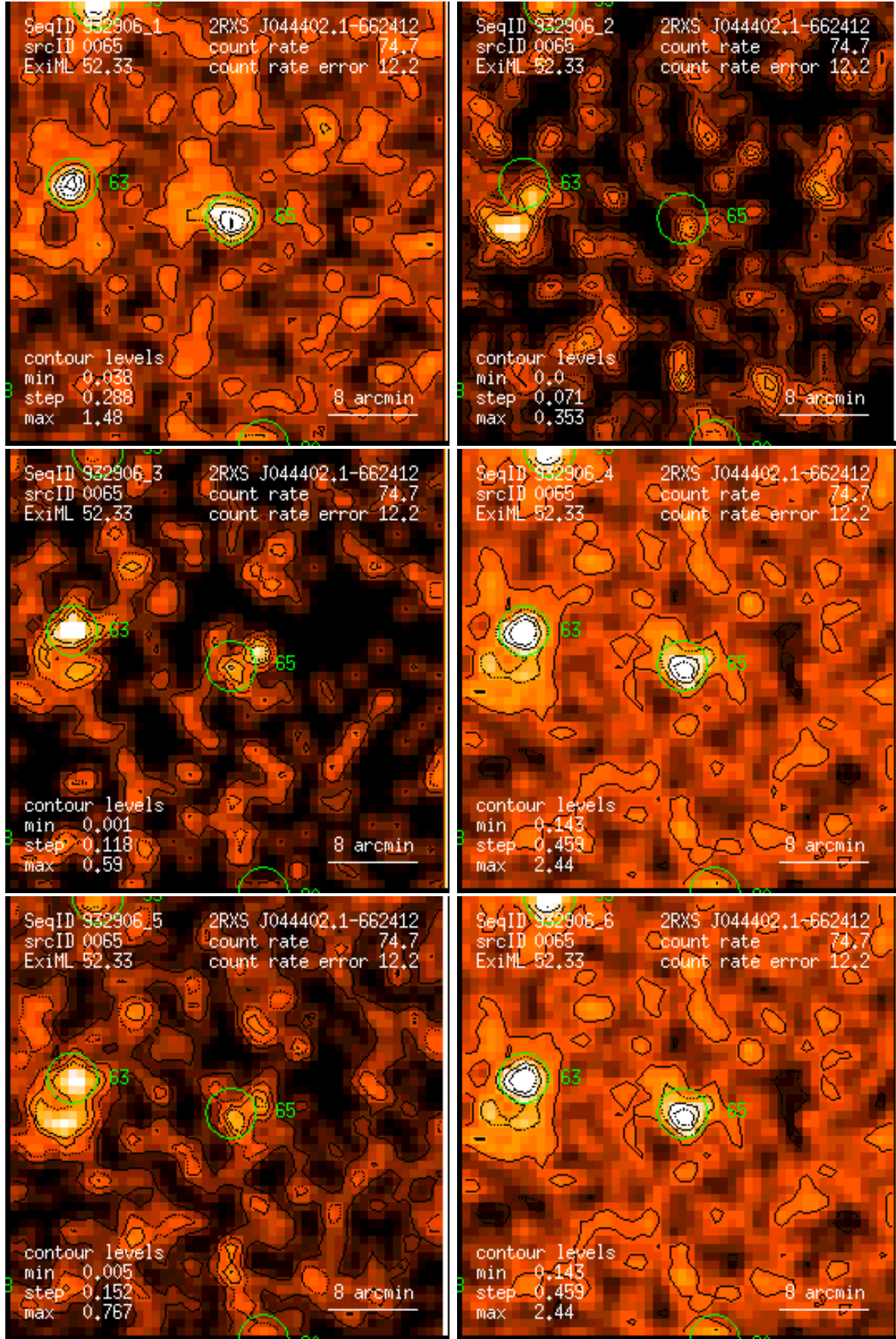
Figure 65: RASS 932906: detection 0065: band rate images, Gaussian filter: (1) PSPC channels 11 – 41, (2) 52 – 90, (3) 91 – 201, (4) 11 – 235, (5) 52 – 201, (6) 11 – 201. Broad band rates in counts/ks. Band rate contour levels in counts/ks/arcmin 2 .
