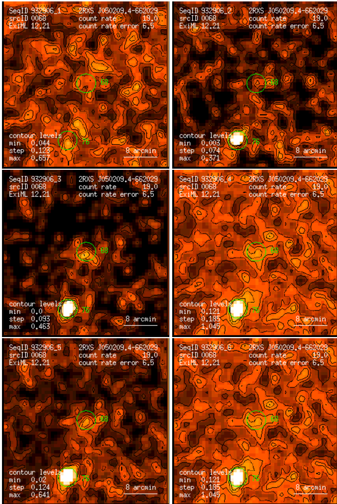
Figure 68: RASS 932906: detection 0068: band rate images, Gaussian filter: (1) PSPC channels 11 – 41, (2) 52 – 90, (3) 91 – 201, (4) 11 – 235, (5) 52 – 201, (6) 11 – 201. Broad band rates in counts/ks. Band rate contour levels in counts/ks/arcmin 2 .
