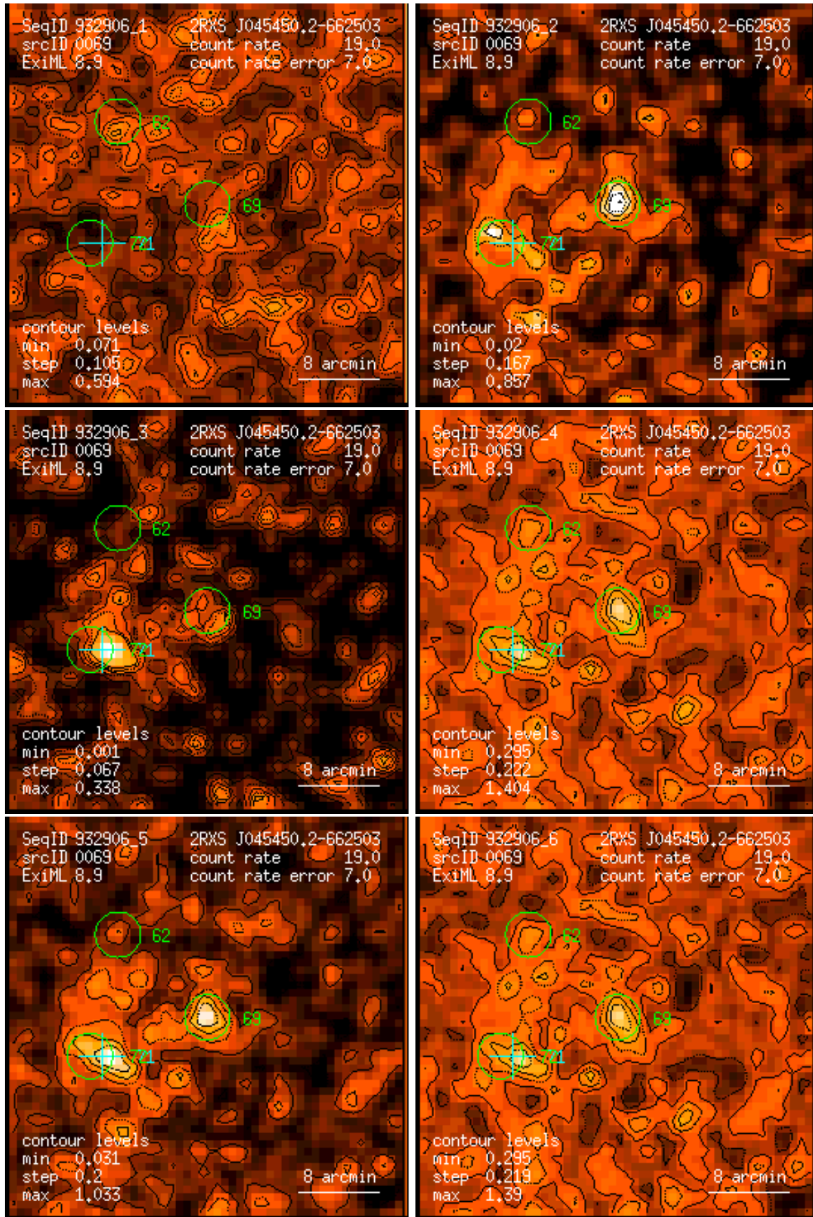
Figure 69: RASS 932906: detection 0069: band rate images, Gaussian filter: (1) PSPC channels 11 – 41, (2) 52 – 90, (3) 91 – 201, (4) 11 – 235, (5) 52 – 201, (6) 11 – 201. Broad band rates in counts/ks. Band rate contour levels in counts/ks/arcmin 2 .
