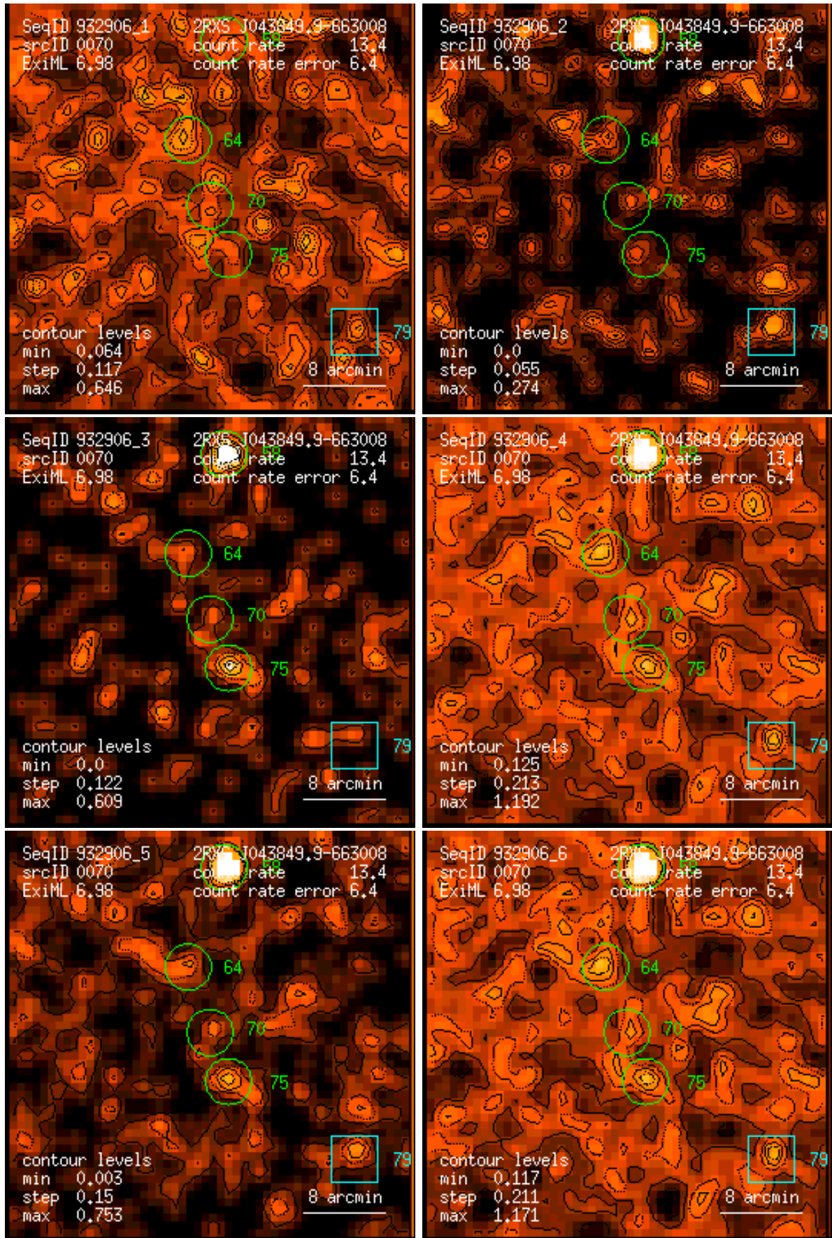
Figure 70: RASS 932906: detection 0070: band rate images, Gaussian filter: (1) PSPC channels 11 – 41, (2) 52 – 90, (3) 91 – 201, (4) 11 – 235, (5) 52 – 201, (6) 11 – 201. Broad band rates in counts/ks. Band rate contour levels in counts/ks/arcmin 2 .
