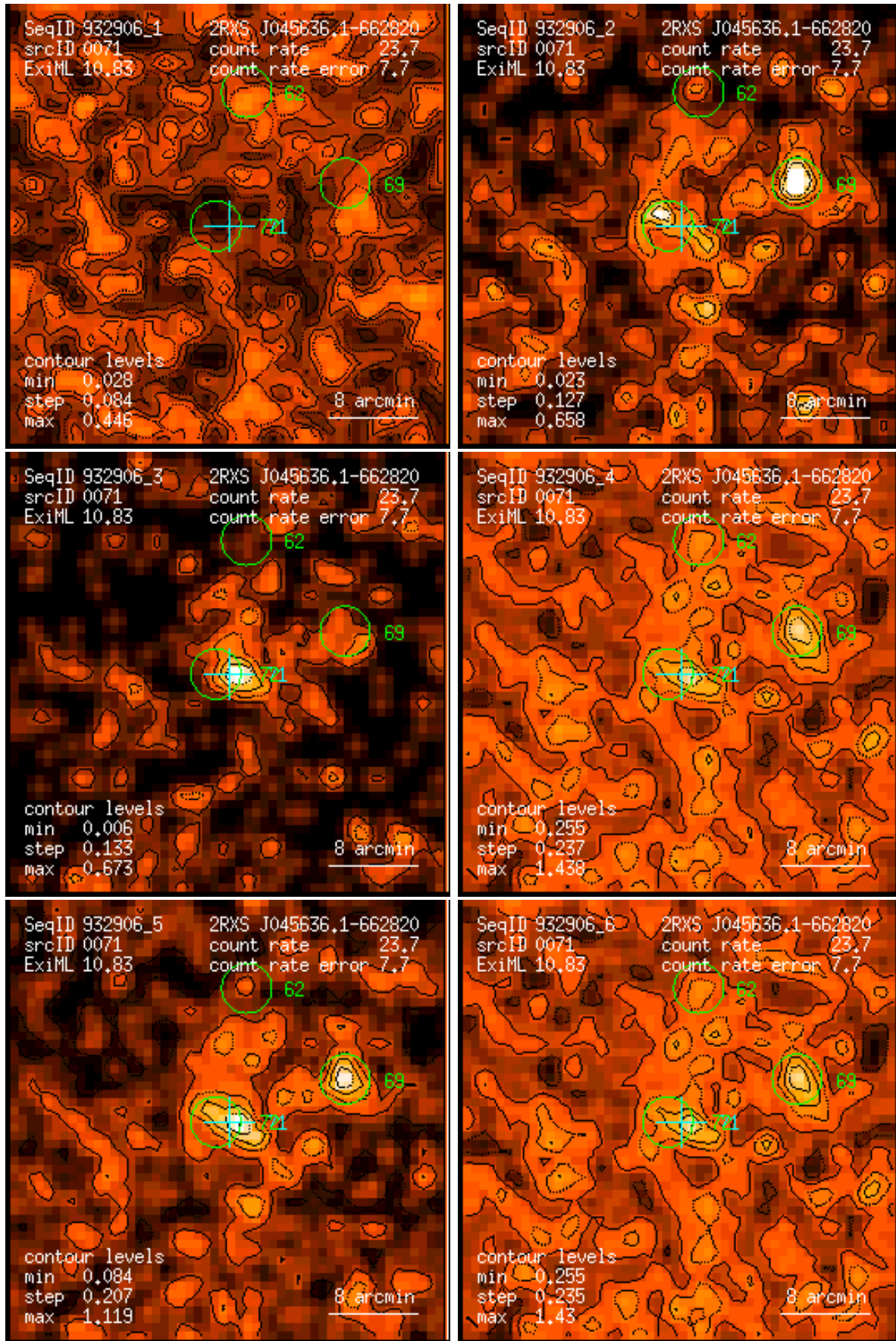
Figure 71: RASS 932906: detection 0071: band rate images, Gaussian filter: (1) PSPC channels 11 – 41, (2) 52 – 90, (3) 91 – 201, (4) 11 – 235, (5) 52 – 201, (6) 11 – 201. Broad band rates in counts/ks. Band rate contour levels in counts/ks/arcmin 2 .
