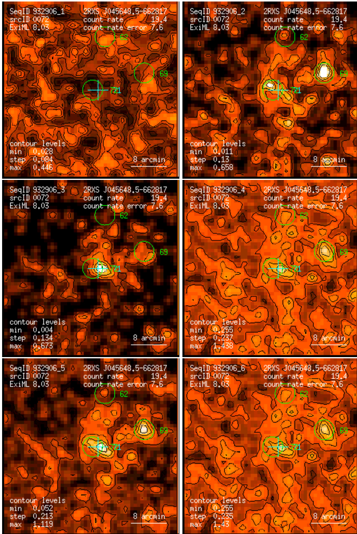
Figure 72: RASS 932906: detection 0072: band rate images, Gaussian filter: (1) PSPC channels 11 – 41, (2) 52 – 90, (3) 91 – 201, (4) 11 – 235, (5) 52 – 201, (6) 11 – 201. Broad band rates in counts/ks. Band rate contour levels in counts/ks/arcmin 2 .
