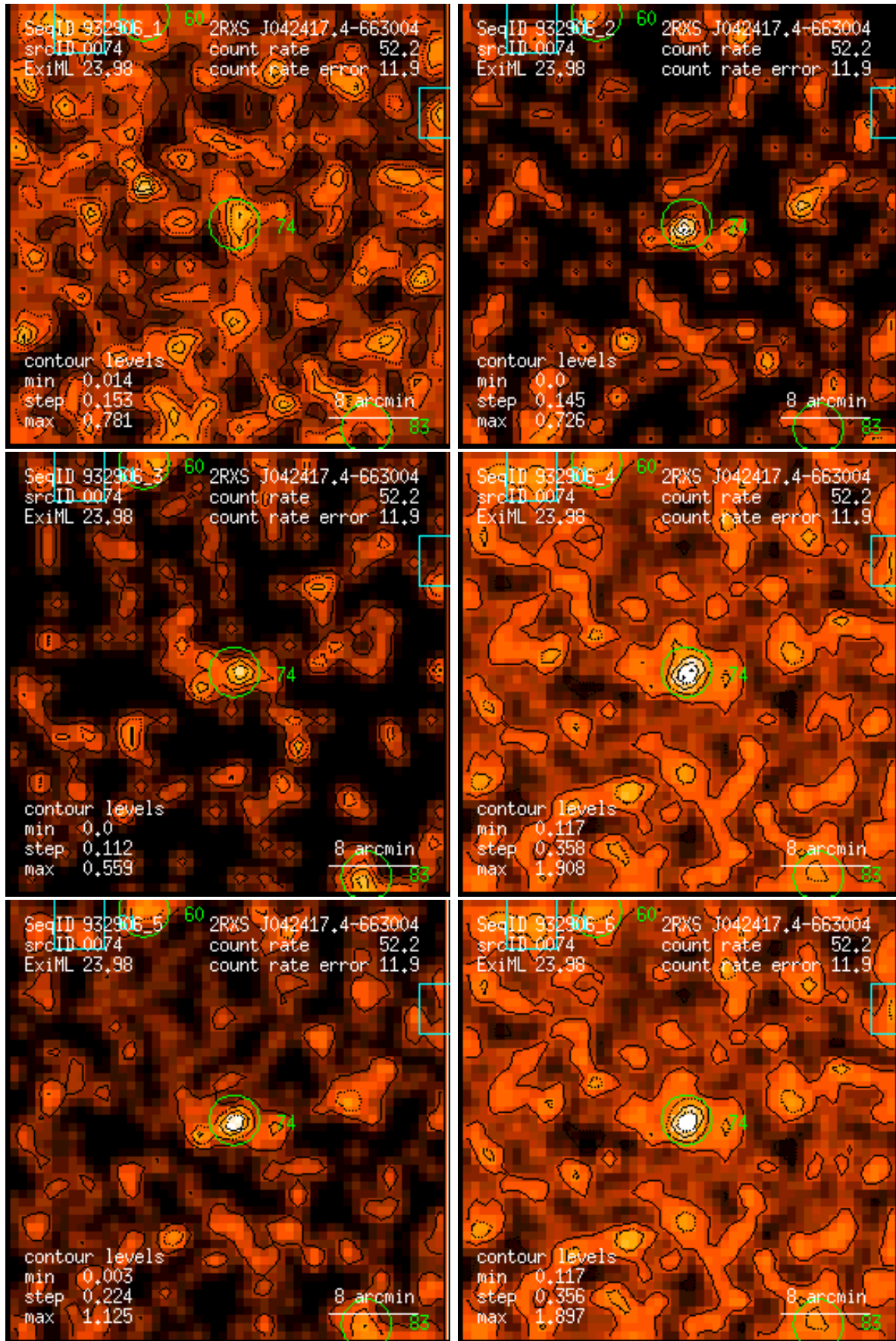
Figure 74: RASS 932906: detection 0074: band rate images, Gaussian filter: (1) PSPC channels 11 – 41, (2) 52 – 90, (3) 91 – 201, (4) 11 – 235, (5) 52 – 201, (6) 11 – 201. Broad band rates in counts/ks. Band rate contour levels in counts/ks/arcmin 2 .
