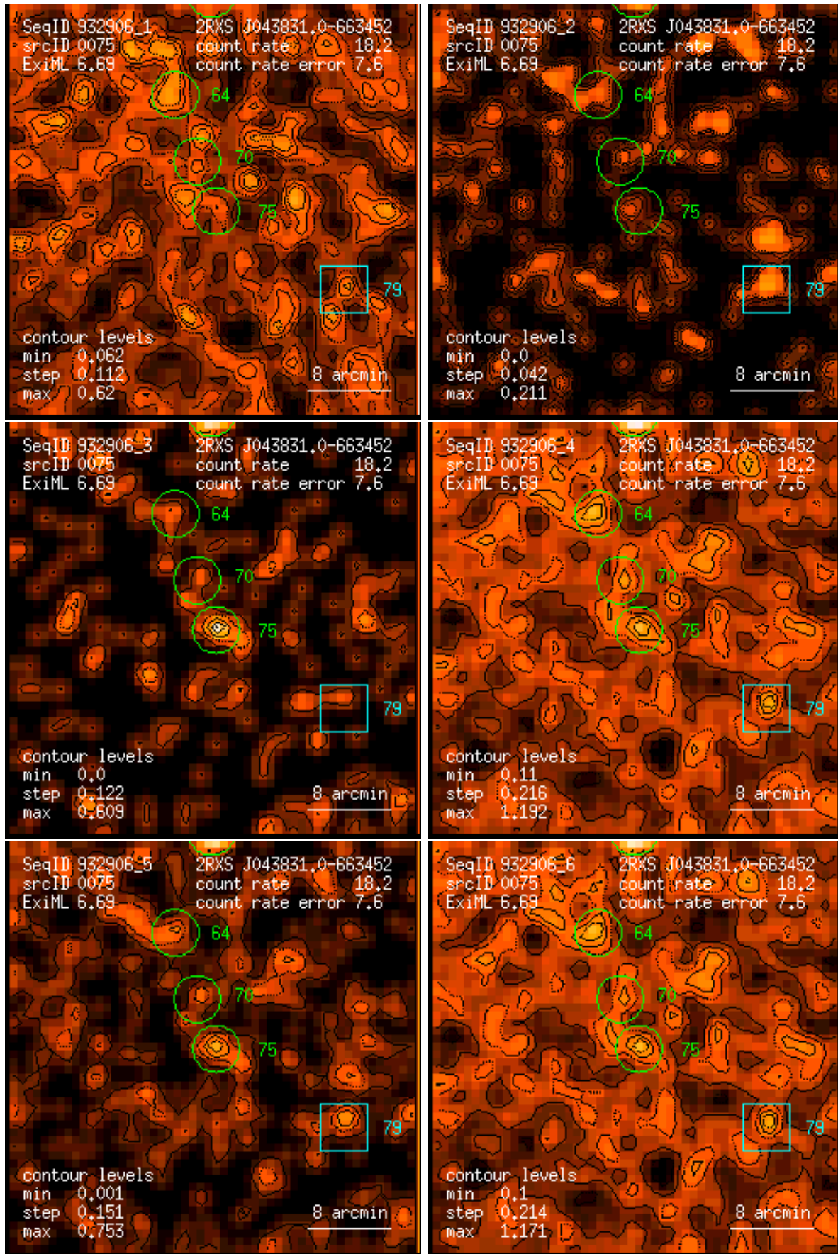
Figure 75: RASS 932906: detection 0075: band rate images, Gaussian filter: (1) PSPC channels 11 – 41, (2) 52 – 90, (3) 91 – 201, (4) 11 – 235, (5) 52 – 201, (6) 11 – 201. Broad band rates in counts/ks. Band rate contour levels in counts/ks/arcmin 2 .
