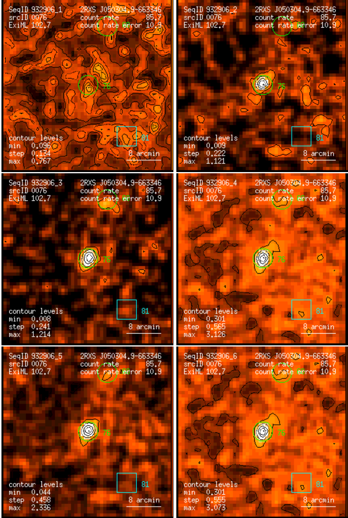
Figure 76: RASS 932906: detection 0076: band rate images, Gaussian filter: (1) PSPC channels 11 – 41, (2) 52 – 90, (3) 91 – 201, (4) 11 – 235, (5) 52 – 201, (6) 11 – 201. Broad band rates in counts/ks. Band rate contour levels in counts/ks/arcmin 2 .
