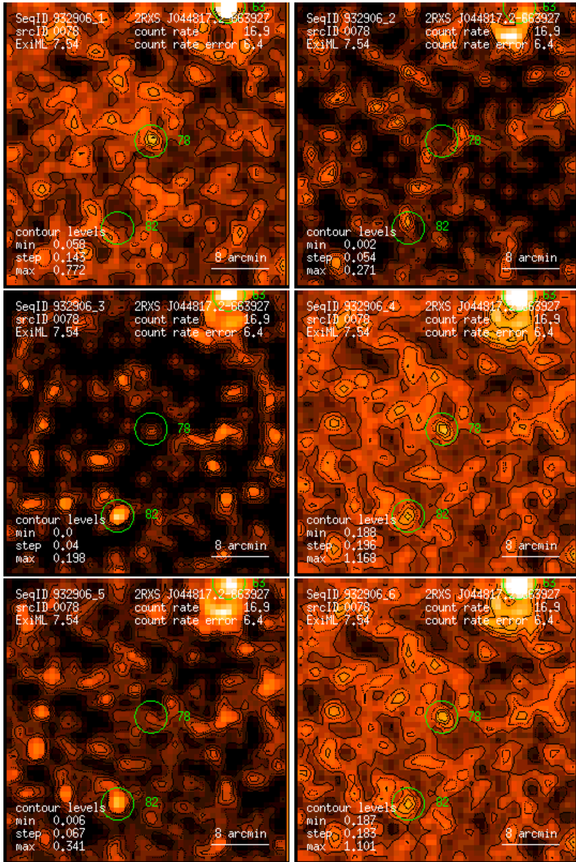
Figure 78: RASS 932906: detection 0078: band rate images, Gaussian filter: (1) PSPC channels 11 – 41, (2) 52 – 90, (3) 91 – 201, (4) 11 – 235, (5) 52 – 201, (6) 11 – 201. Broad band rates in counts/ks. Band rate contour levels in counts/ks/arcmin 2 .
