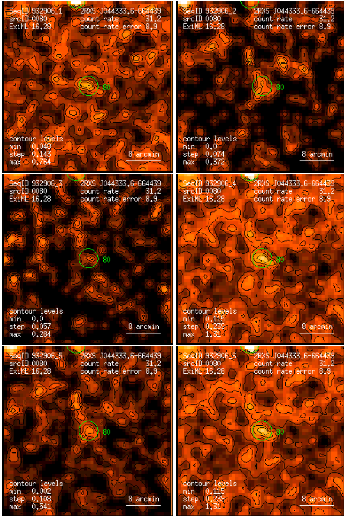
Figure 80: RASS 932906: detection 0080: band rate images, Gaussian filter: (1) PSPC channels 11 – 41, (2) 52 – 90, (3) 91 – 201, (4) 11 – 235, (5) 52 – 201, (6) 11 – 201. Broad band rates in counts/ks. Band rate contour levels in counts/ks/arcmin 2 .
