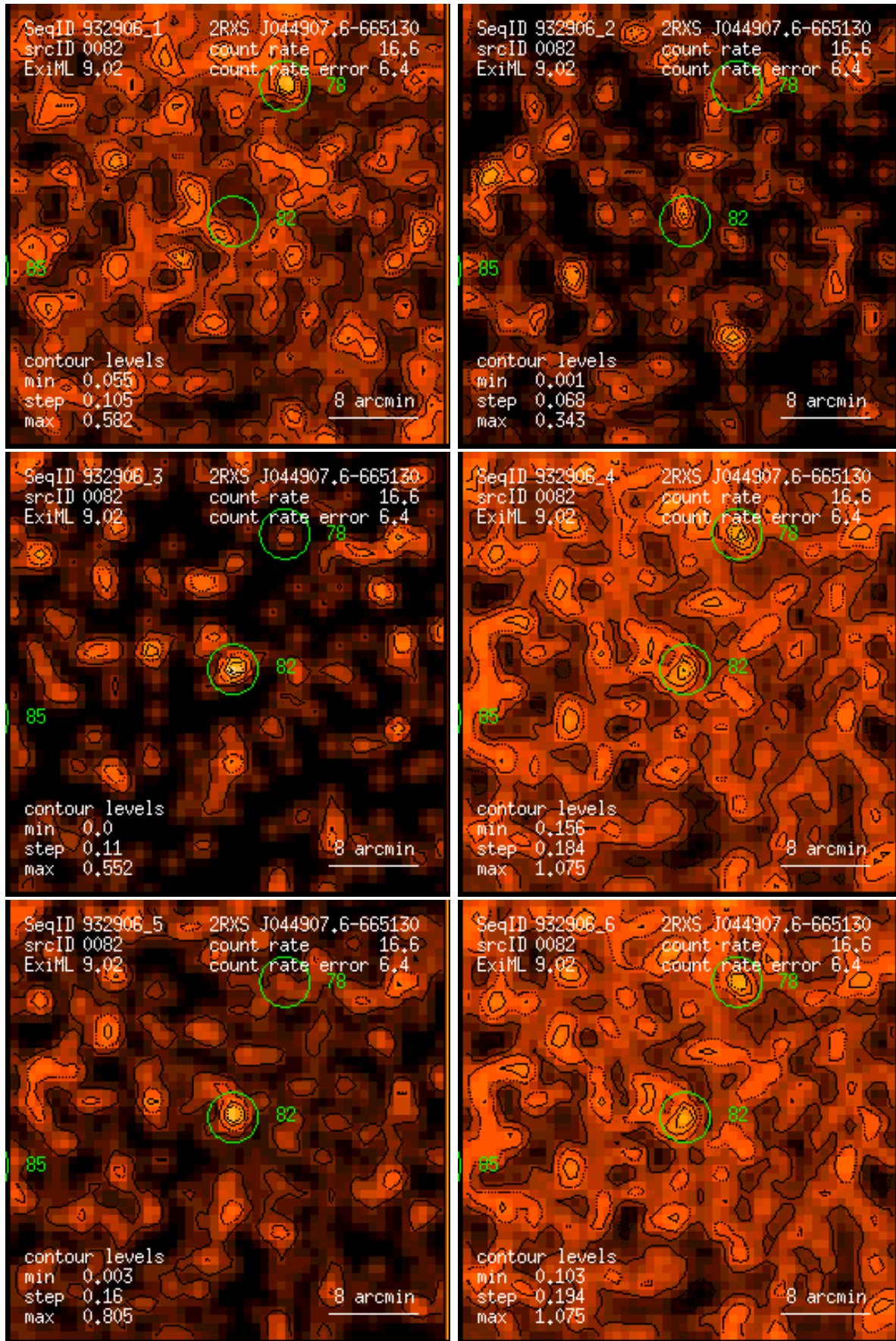
Figure 82: RASS 932906: detection 0082: band rate images, Gaussian filter: (1) PSPC channels 11 – 41, (2) 52 – 90, (3) 91 – 201, (4) 11 – 235, (5) 52 – 201, (6) 11 – 201. Broad band rates in counts/ks. Band rate contour levels in counts/ks/arcmin 2 .
