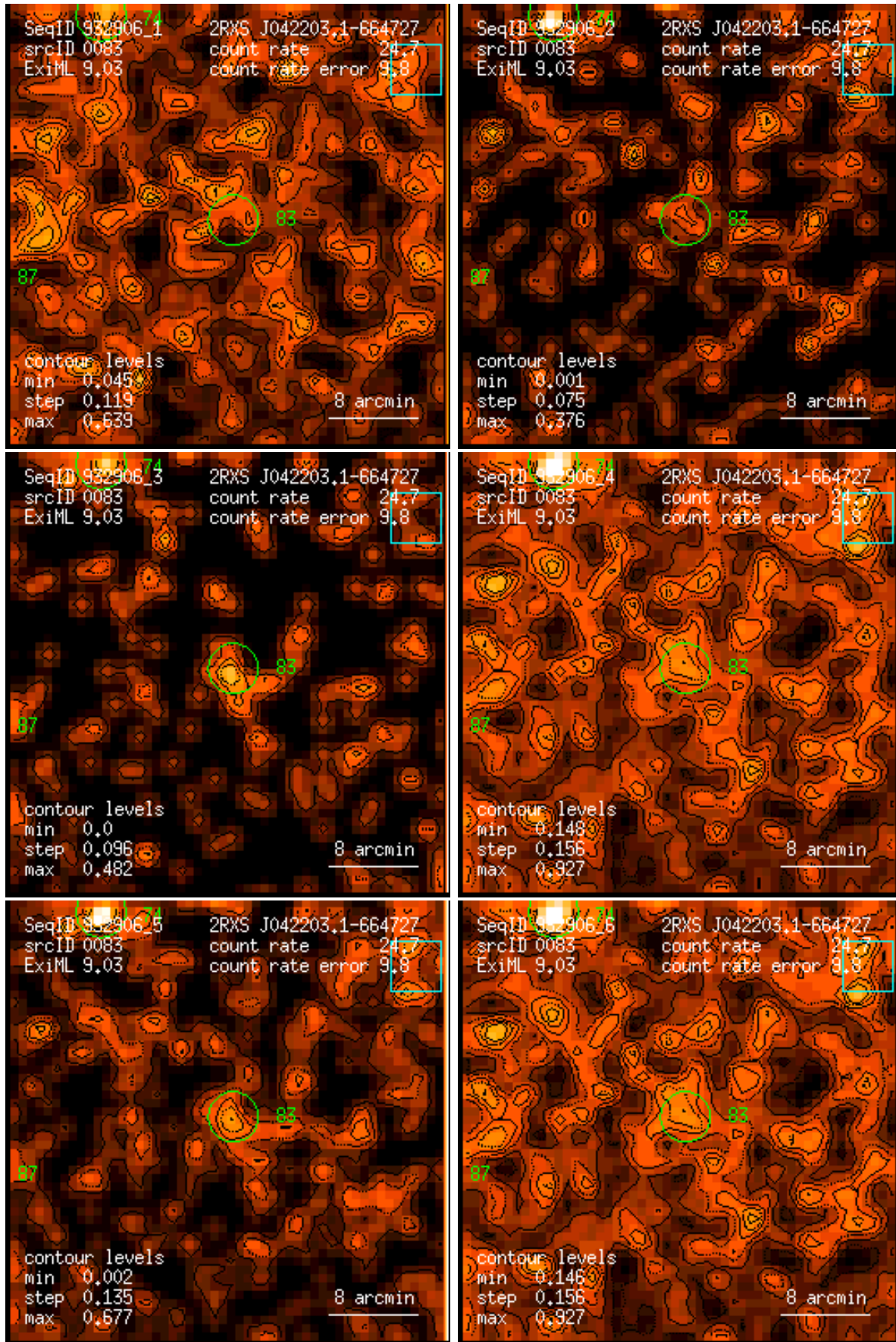
Figure 83: RASS 932906: detection 0083: band rate images, Gaussian filter: (1) PSPC channels 11 – 41, (2) 52 – 90, (3) 91 – 201, (4) 11 – 235, (5) 52 – 201, (6) 11 – 201. Broad band rates in counts/ks. Band rate contour levels in counts/ks/arcmin 2 .
