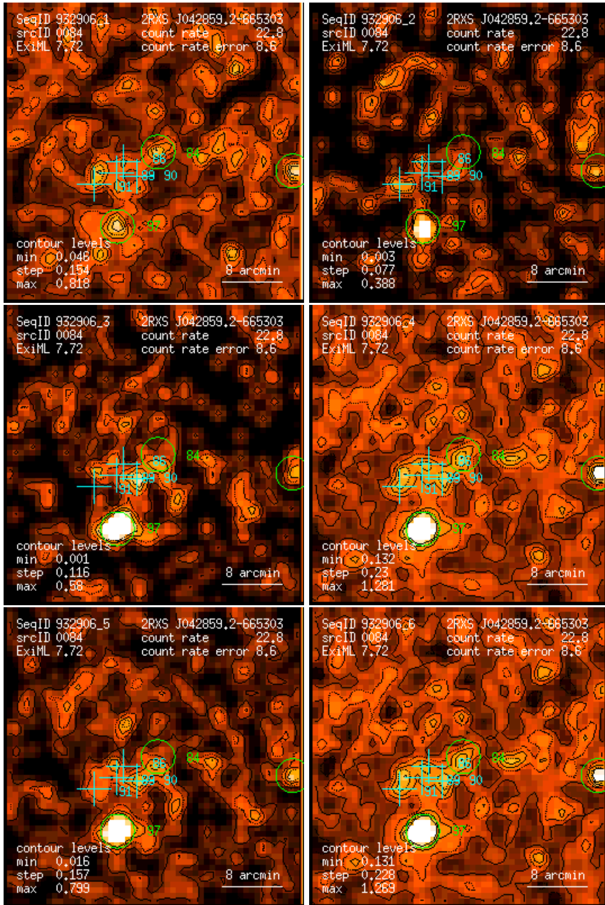
Figure 84: RASS 932906: detection 0084: band rate images, Gaussian filter: (1) PSPC channels 11 – 41, (2) 52 – 90, (3) 91 – 201, (4) 11 – 235, (5) 52 – 201, (6) 11 – 201. Broad band rates in counts/ks. Band rate contour levels in counts/ks/arcmin 2 .
