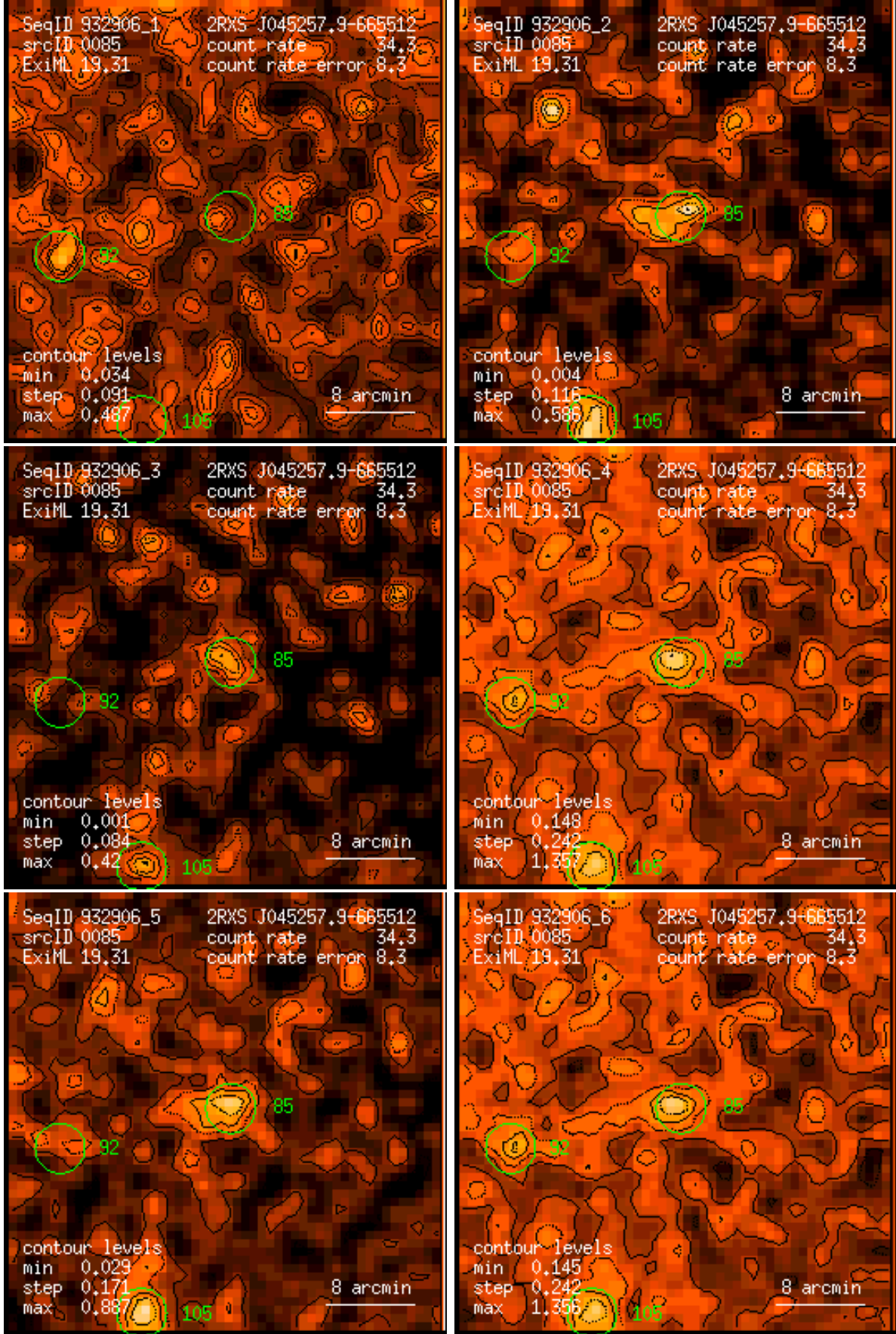
Figure 85: RASS 932906: detection 0085: band rate images, Gaussian filter: (1) PSPC channels 11 – 41, (2) 52 – 90, (3) 91 – 201, (4) 11 – 235, (5) 52 – 201, (6) 11 – 201. Broad band rates in counts/ks. Band rate contour levels in counts/ks/arcmin 2 .
