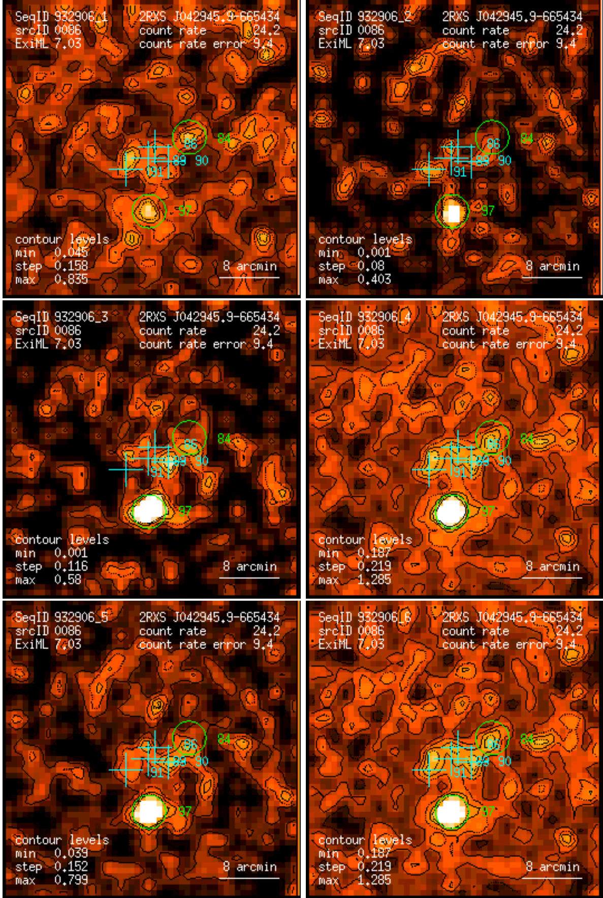
Figure 86: RASS 932906: detection 0086: band rate images, Gaussian filter: (1) PSPC channels 11 – 41, (2) 52 – 90, (3) 91 – 201, (4) 11 – 235, (5) 52 – 201, (6) 11 – 201. Broad band rates in counts/ks. Band rate contour levels in counts/ks/arcmin 2 .
