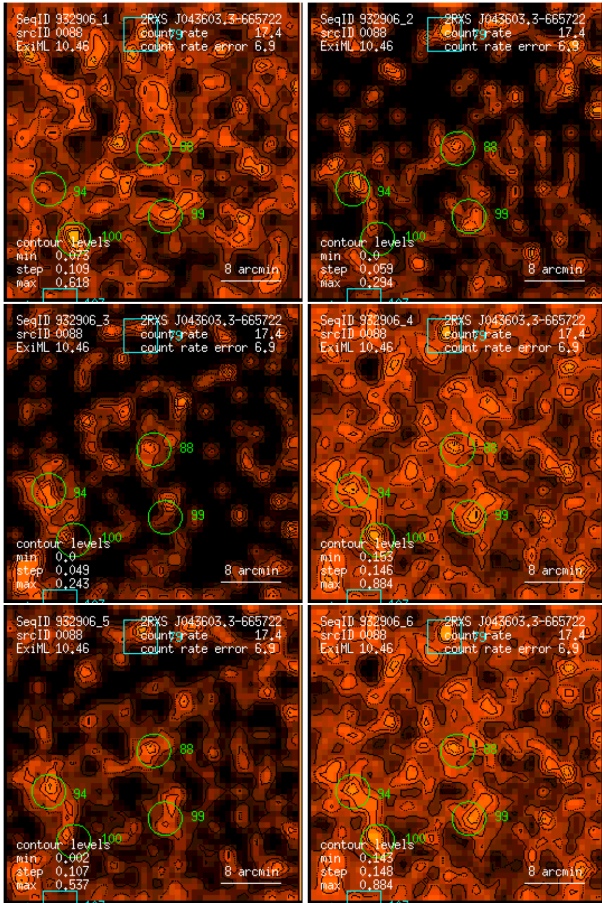
Figure 88: RASS 932906: detection 0088: band rate images, Gaussian filter: (1) PSPC channels 11 – 41, (2) 52 – 90, (3) 91 – 201, (4) 11 – 235, (5) 52 – 201, (6) 11 – 201. Broad band rates in counts/ks. Band rate contour levels in counts/ks/arcmin 2 .
