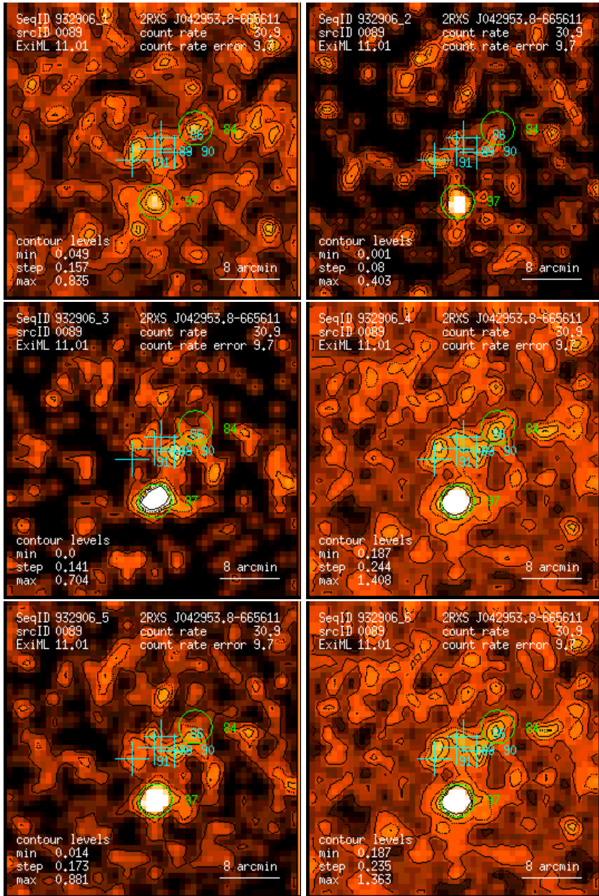
Figure 89: RASS 932906: detection 0089: band rate images, Gaussian filter: (1) PSPC channels 11 – 41, (2) 52 – 90, (3) 91 – 201, (4) 11 – 235, (5) 52 – 201, (6) 11 – 201. Broad band rates in counts/ks. Band rate contour levels in counts/ks/arcmin 2 .
