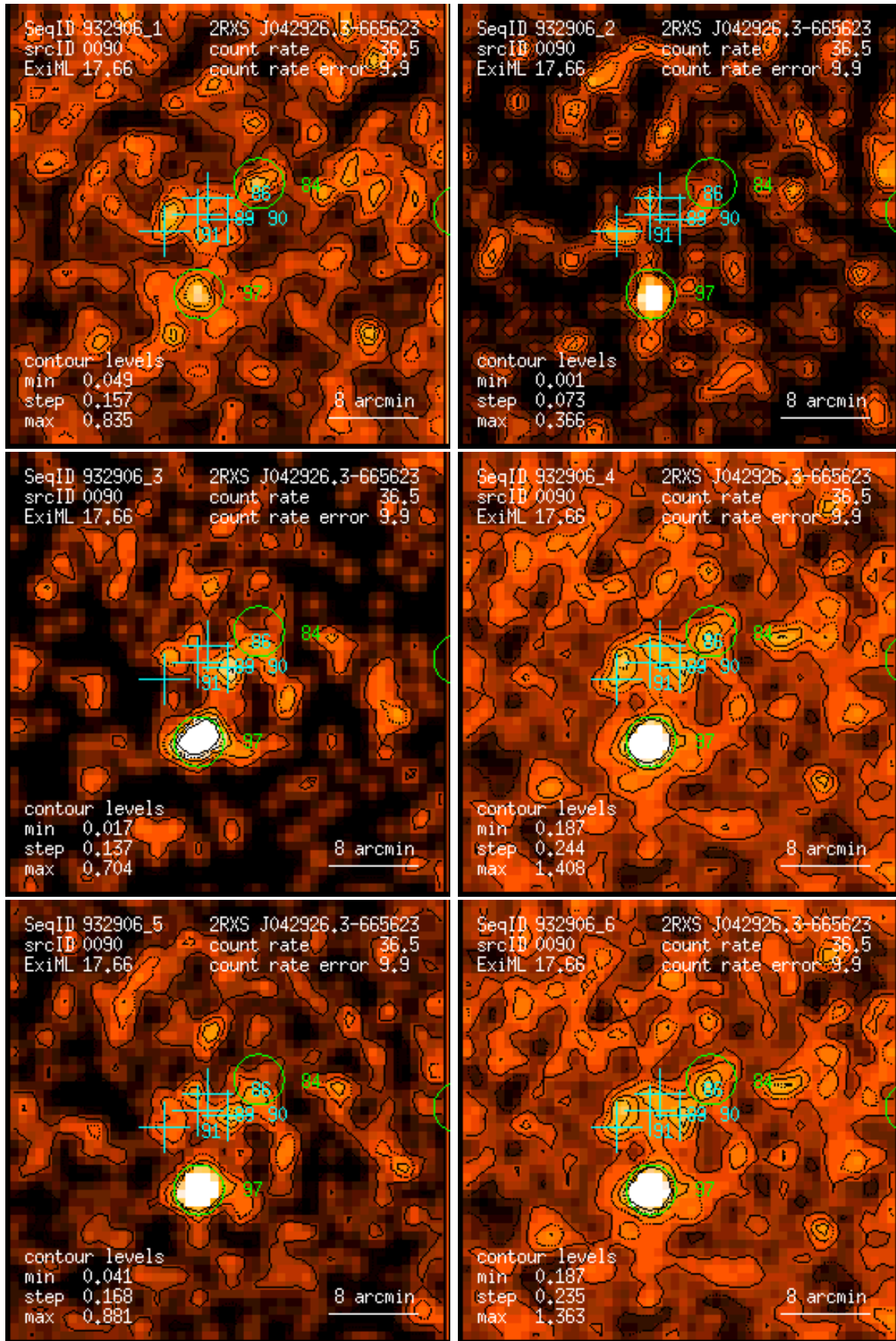
Figure 90: RASS 932906: detection 0090: band rate images, Gaussian filter: (1) PSPC channels 11 – 41, (2) 52 – 90, (3) 91 – 201, (4) 11 – 235, (5) 52 – 201, (6) 11 – 201. Broad band rates in counts/ks. Band rate contour levels in counts/ks/arcmin 2 .
