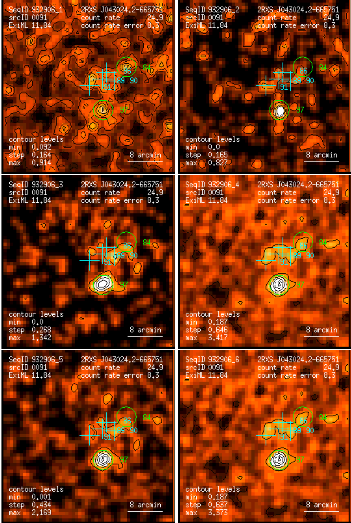
Figure 91: RASS 932906: detection 0091: band rate images, Gaussian filter: (1) PSPC channels 11 – 41, (2) 52 – 90, (3) 91 – 201, (4) 11 – 235, (5) 52 – 201, (6) 11 – 201. Broad band rates in counts/ks. Band rate contour levels in counts/ks/arcmin 2 .
