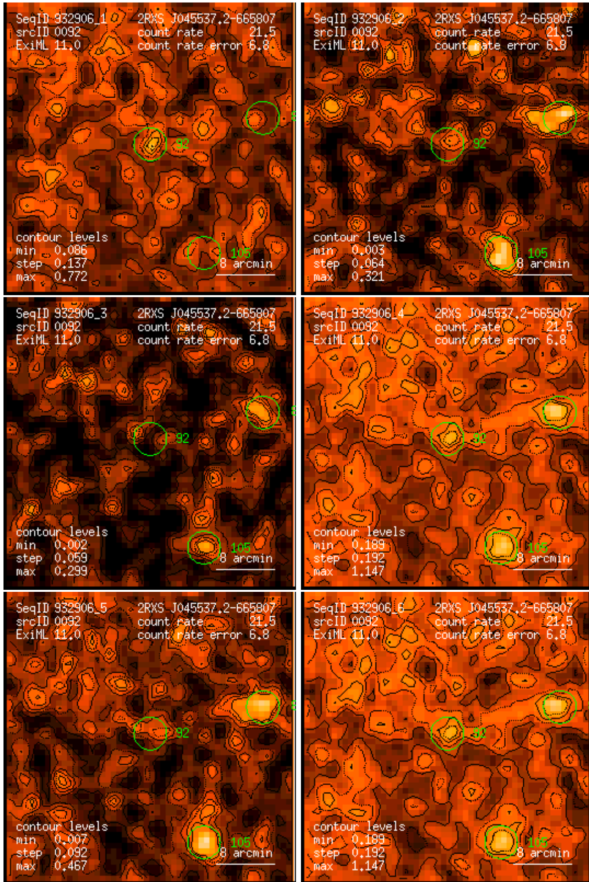
Figure 92: RASS 932906: detection 0092: band rate images, Gaussian filter: (1) PSPC channels 11 – 41, (2) 52 – 90, (3) 91 – 201, (4) 11 – 235, (5) 52 – 201, (6) 11 – 201. Broad band rates in counts/ks. Band rate contour levels in counts/ks/arcmin 2 .
