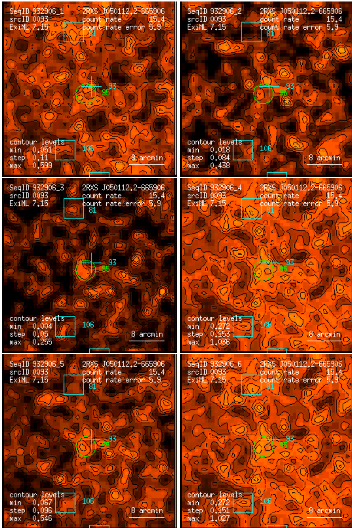
Figure 93: RASS 932906: detection 0093: band rate images, Gaussian filter: (1) PSPC channels 11 – 41, (2) 52 – 90, (3) 91 – 201, (4) 11 – 235, (5) 52 – 201, (6) 11 – 201. Broad band rates in counts/ks. Band rate contour levels in counts/ks/arcmin 2 .
