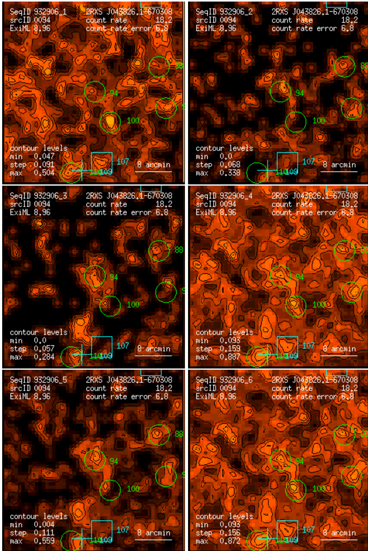
Figure 94: RASS 932906: detection 0094: band rate images, Gaussian filter: (1) PSPC channels 11 – 41, (2) 52 – 90, (3) 91 – 201, (4) 11 – 235, (5) 52 – 201, (6) 11 – 201. Broad band rates in counts/ks. Band rate contour levels in counts/ks/arcmin 2 .
