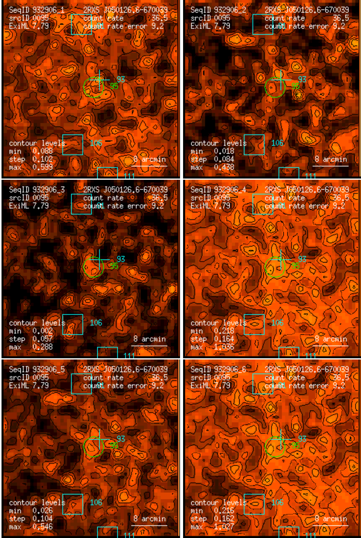
Figure 95: RASS 932906: detection 0095: band rate images, Gaussian filter: (1) PSPC channels 11 – 41, (2) 52 – 90, (3) 91 – 201, (4) 11 – 235, (5) 52 – 201, (6) 11 – 201. Broad band rates in counts/ks. Band rate contour levels in counts/ks/arcmin 2 .
