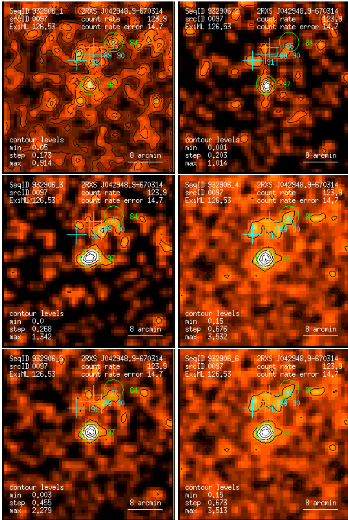
Figure 97: RASS 932906: detection 0097: band rate images, Gaussian filter: (1) PSPC channels 11 – 41, (2) 52 – 90, (3) 91 – 201, (4) 11 – 235, (5) 52 – 201, (6) 11 – 201. Broad band rates in counts/ks. Band rate contour levels in counts/ks/arcmin 2 .
