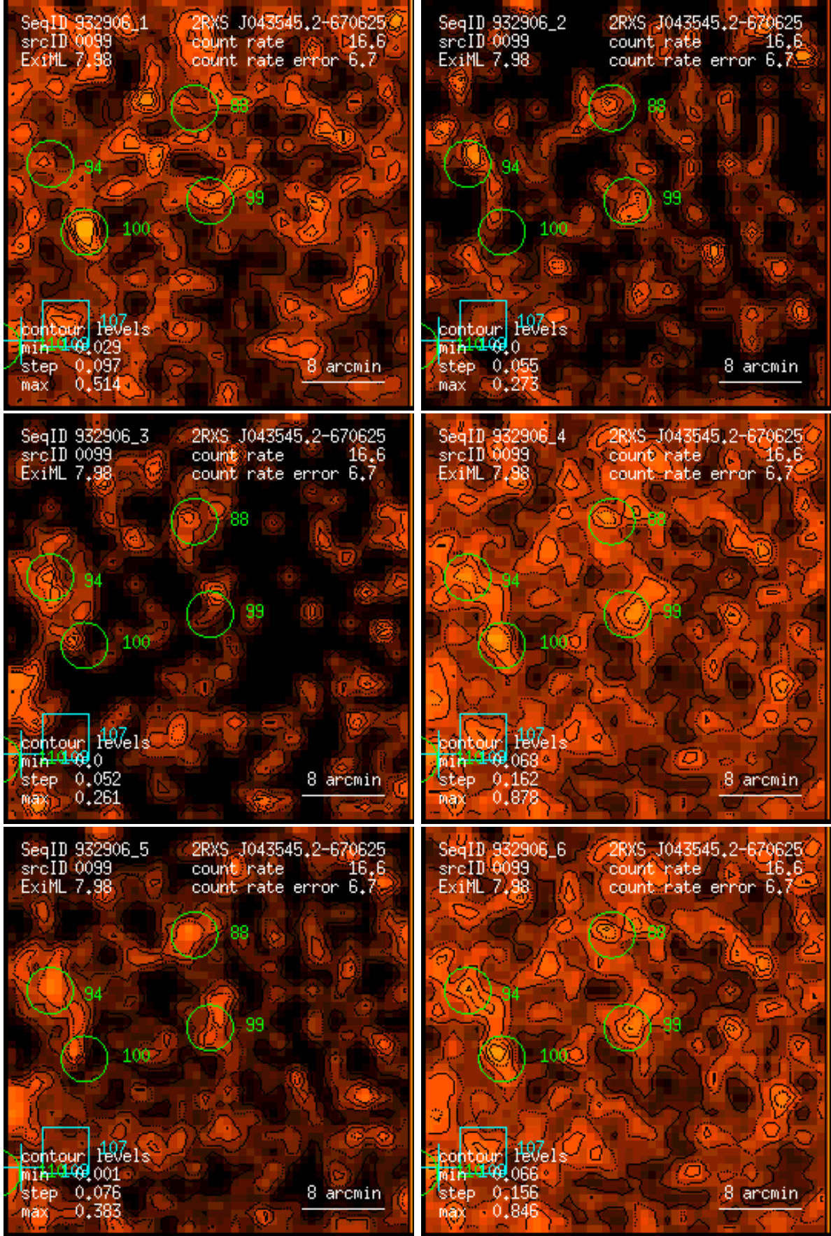
Figure 99: RASS 932906: detection 0099: band rate images, Gaussian filter: (1) PSPC channels 11 – 41, (2) 52 – 90, (3) 91 – 201, (4) 11 – 235, (5) 52 – 201, (6) 11 – 201. Broad band rates in counts/ks. Band rate contour levels in counts/ks/arcmin 2 .
