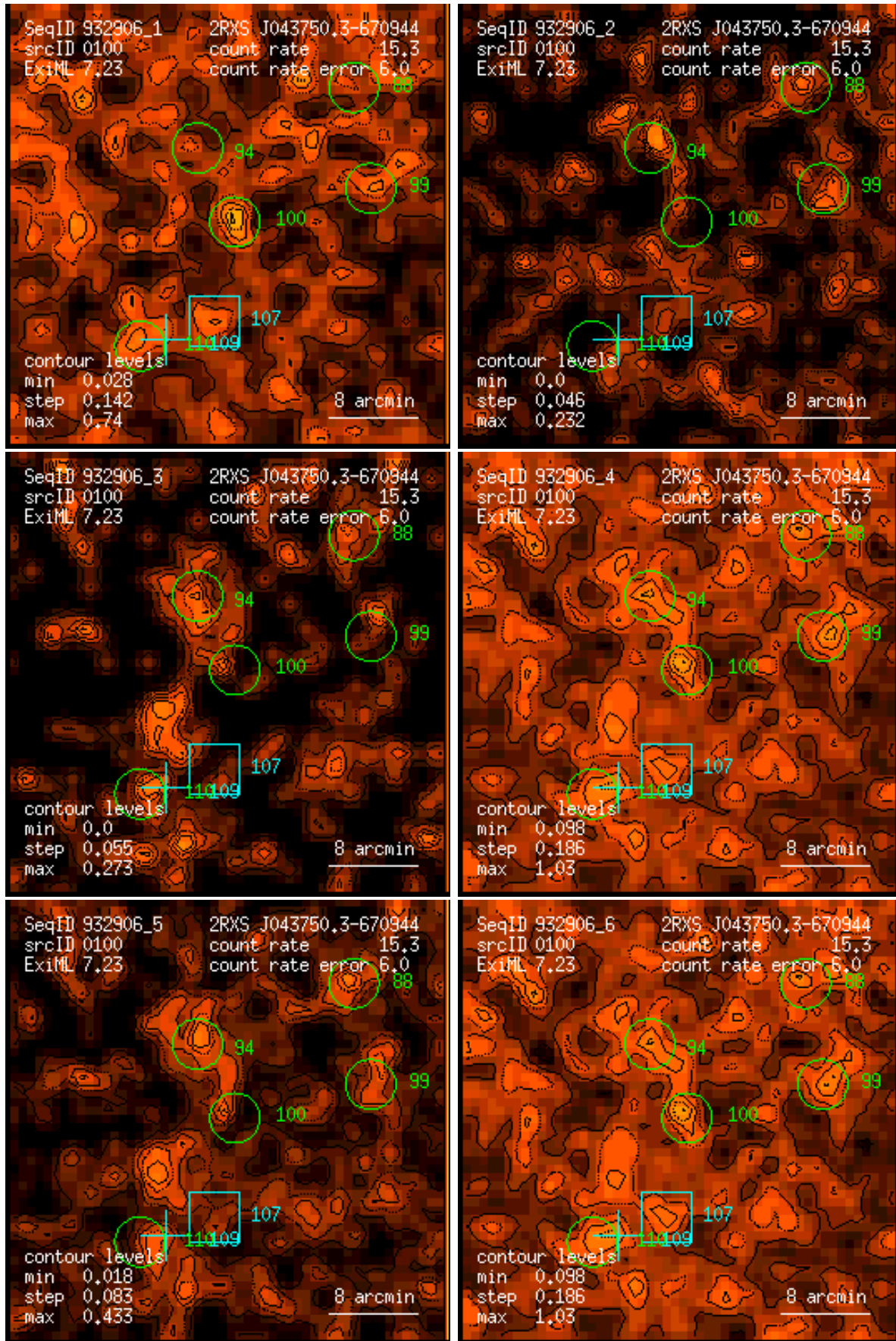
Figure 100: RASS 932906: detection 0100: band rate images, Gaussian filter: (1) PSPC channels 11 – 41, (2) 52 – 90, (3) 91 – 201, (4) 11 – 235, (5) 52 – 201, (6) 11 – 201. Broad band rates in counts/ks. Band rate contour levels in counts/ks/arcmin 2 .
