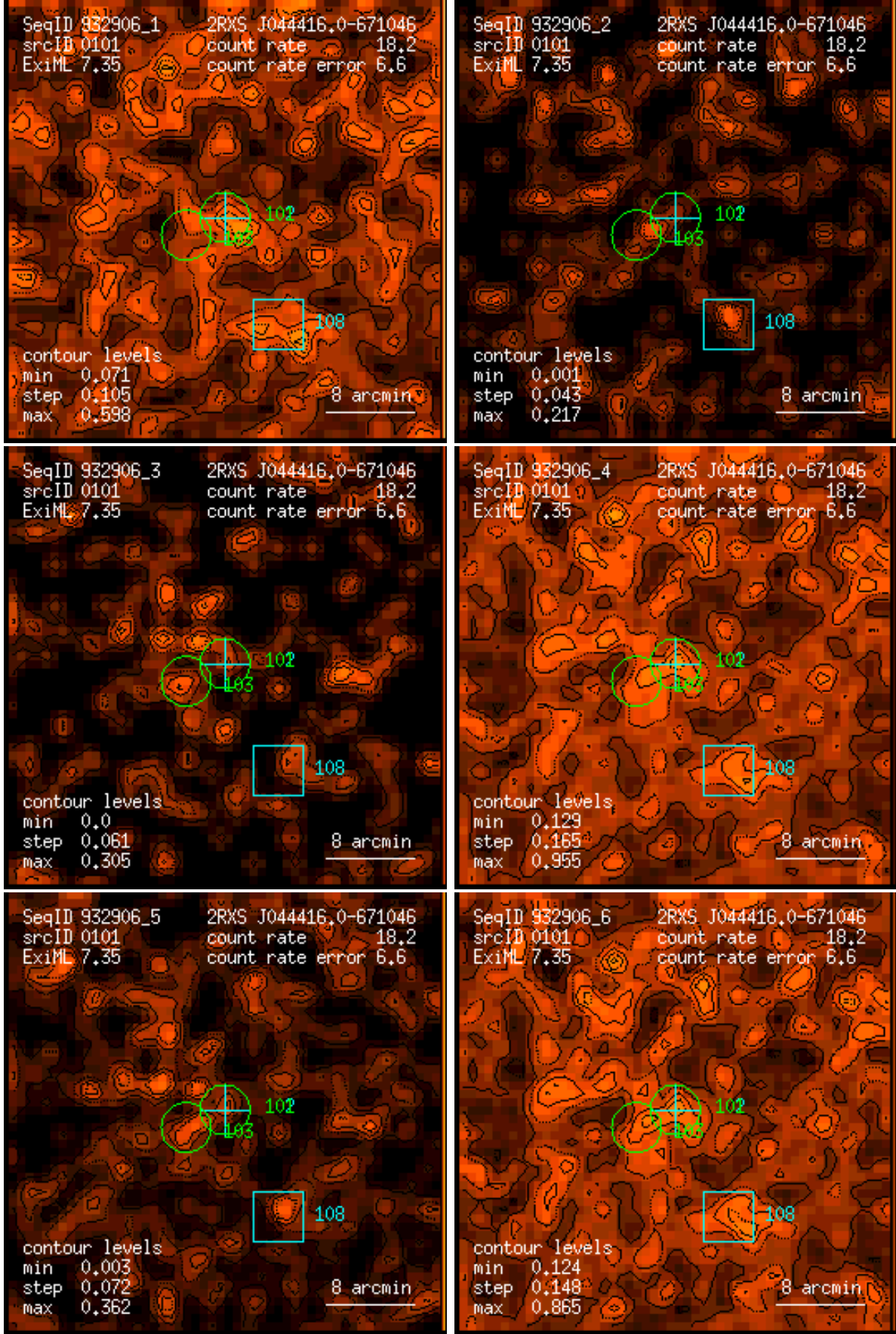
Figure 101: RASS 932906: detection 0101: band rate images, Gaussian filter: (1) PSPC channels 11 – 41, (2) 52 – 90, (3) 91 – 201, (4) 11 – 235, (5) 52 – 201, (6) 11 – 201. Broad band rates in counts/ks. Band rate contour levels in counts/ks/arcmin 2 .
