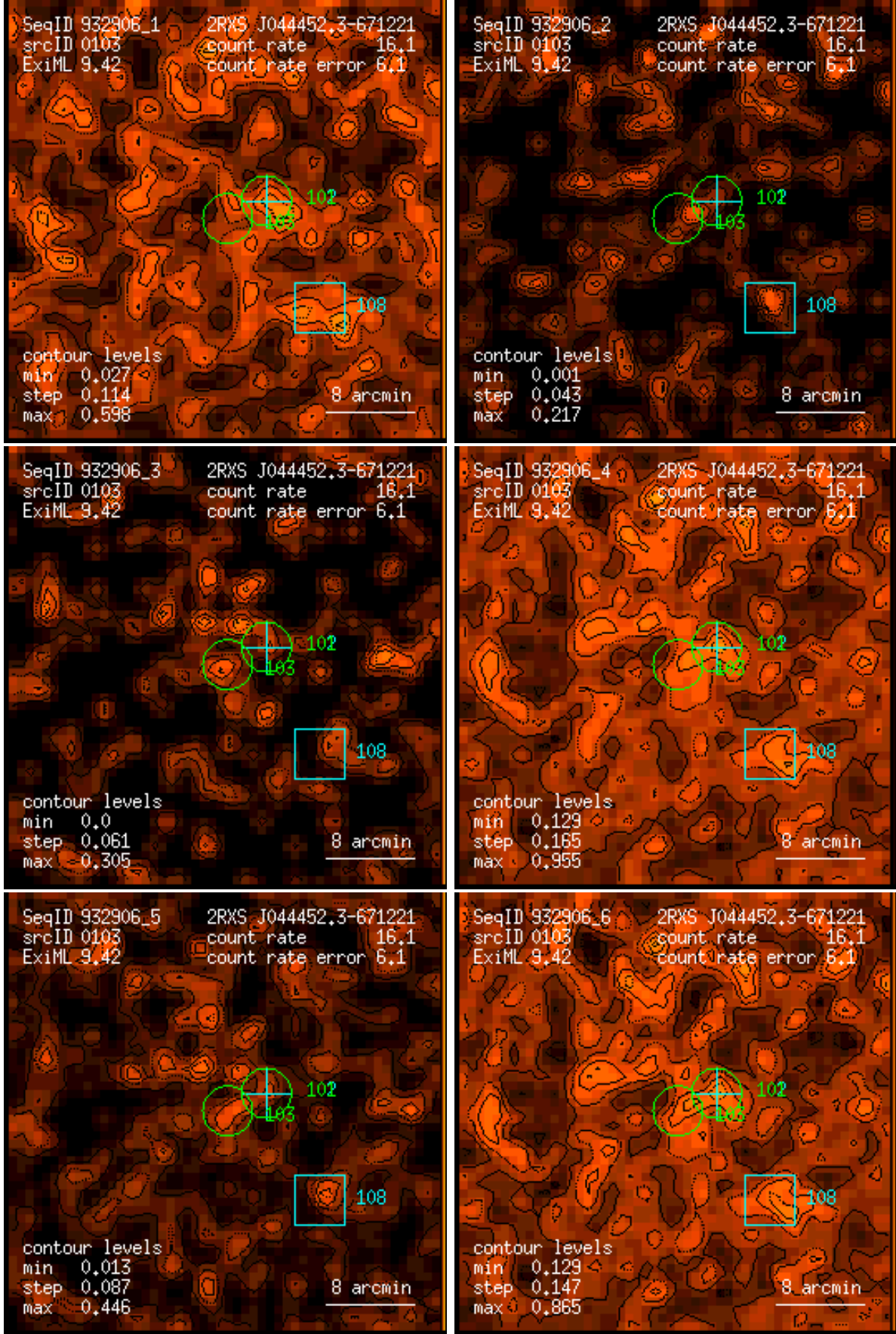
Figure 103: RASS 932906: detection 0103: band rate images, Gaussian filter: (1) PSPC channels 11 – 41, (2) 52 – 90, (3) 91 – 201, (4) 11 – 235, (5) 52 – 201, (6) 11 – 201. Broad band rates in counts/ks. Band rate contour levels in counts/ks/arcmin 2 .
