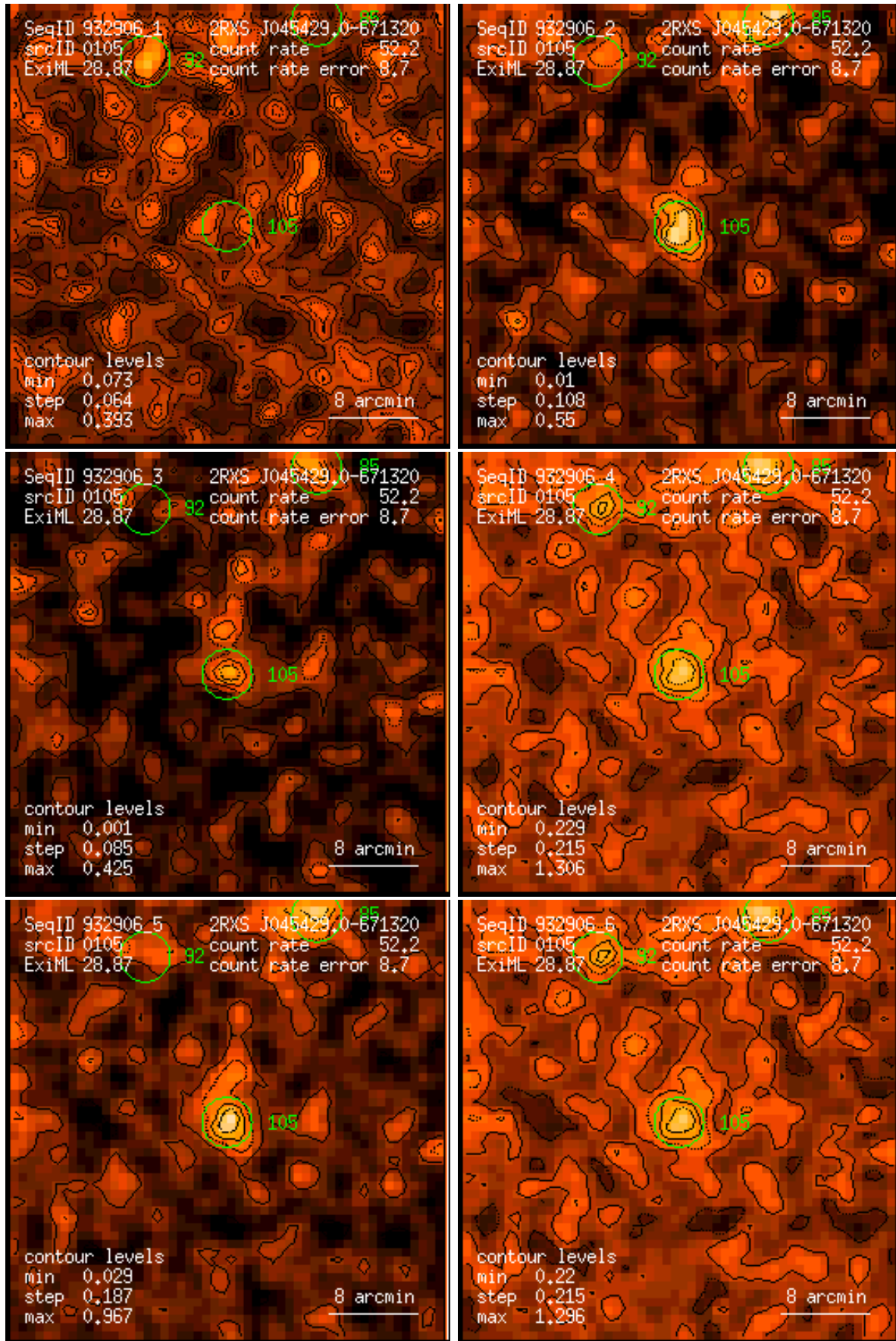
Figure 105: RASS 932906: detection 0105: band rate images, Gaussian filter: (1) PSPC channels 11 – 41, (2) 52 – 90, (3) 91 – 201, (4) 11 – 235, (5) 52 – 201, (6) 11 – 201. Broad band rates in counts/ks. Band rate contour levels in counts/ks/arcmin 2 .
