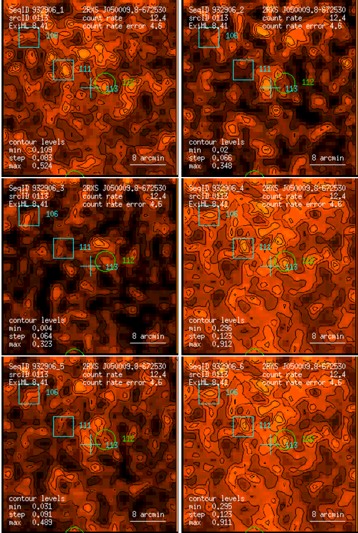
Figure 113: RASS 932906: detection 0113: band rate images, Gaussian filter: (1) PSPC channels 11 – 41, (2) 52 – 90, (3) 91 – 201, (4) 11 – 235, (5) 52 – 201, (6) 11 – 201. Broad band rates in counts/ks. Band rate contour levels in counts/ks/arcmin 2 .
