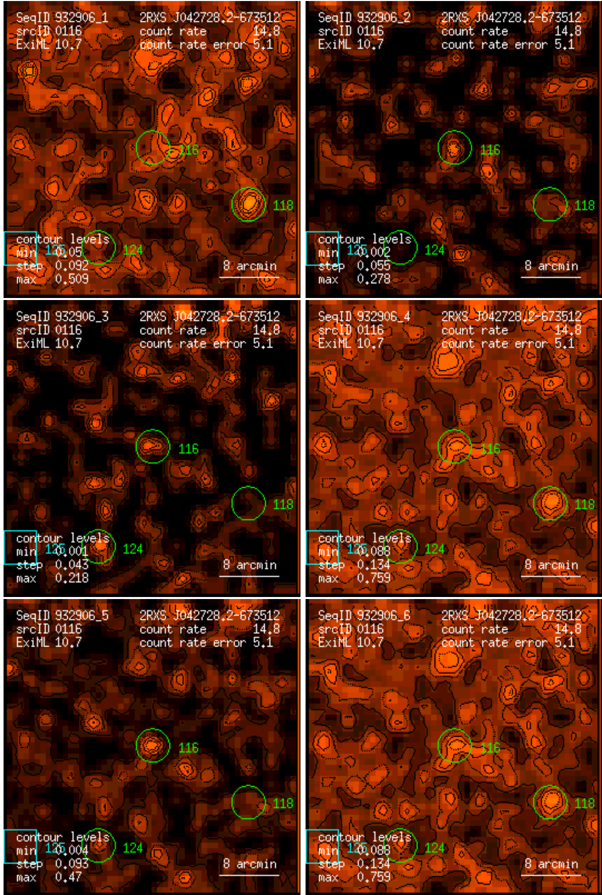
Figure 116: RASS 932906: detection 0116: band rate images, Gaussian filter: (1) PSPC channels 11 – 41, (2) 52 – 90, (3) 91 – 201, (4) 11 – 235, (5) 52 – 201, (6) 11 – 201. Broad band rates in counts/ks. Band rate contour levels in counts/ks/arcmin 2 .
