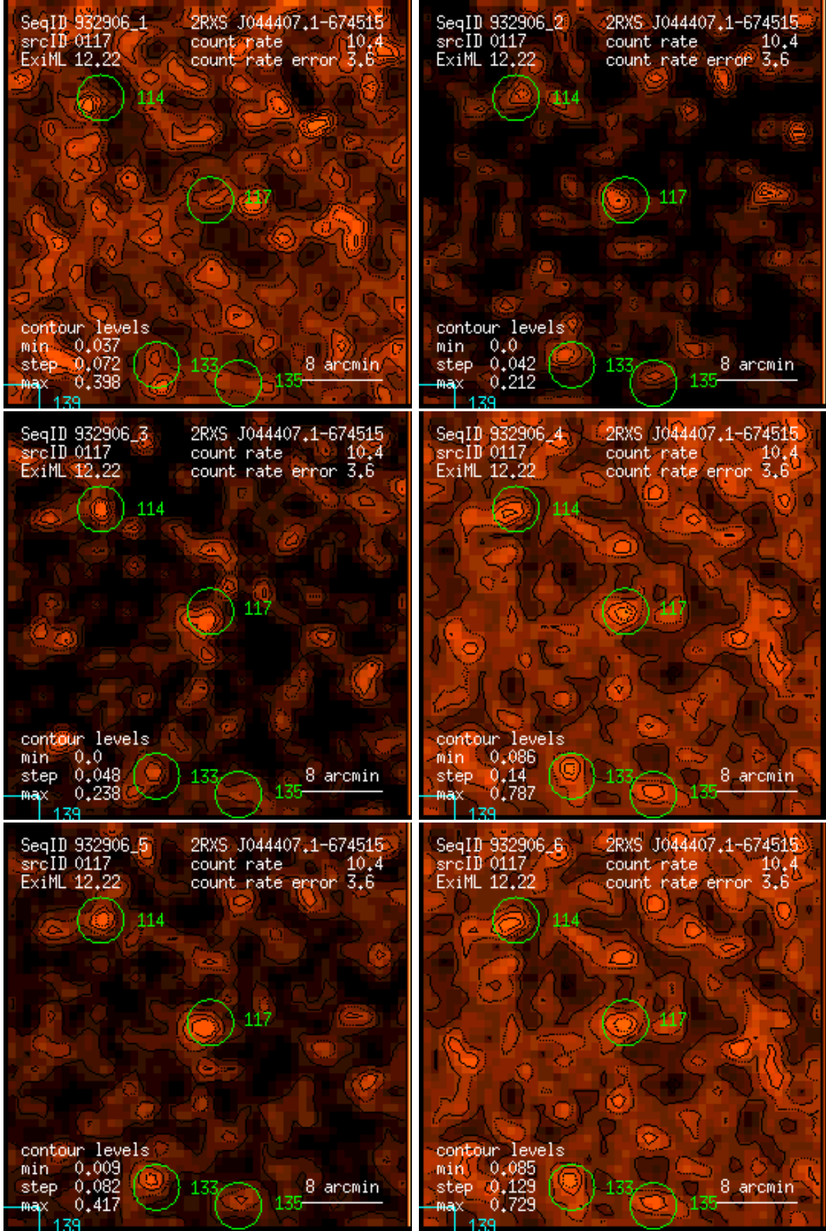
Figure 117: RASS 932906: detection 0117: band rate images, Gaussian filter: (1) PSPC channels 11 – 41, (2) 52 – 90, (3) 91 – 201, (4) 11 – 235, (5) 52 – 201, (6) 11 – 201. Broad band rates in counts/ks. Band rate contour levels in counts/ks/arcmin 2 .
