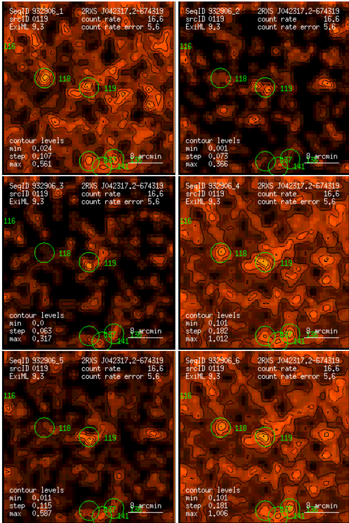
Figure 119: RASS 932906: detection 0119: band rate images, Gaussian filter: (1) PSPC channels 11 – 41, (2) 52 – 90, (3) 91 – 201, (4) 11 – 235, (5) 52 – 201, (6) 11 – 201. Broad band rates in counts/ks. Band rate contour levels in counts/ks/arcmin 2 .
