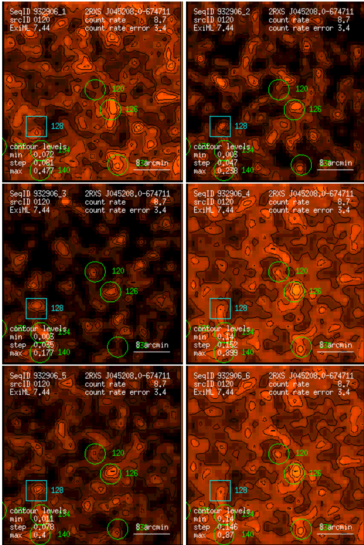
Figure 120: RASS 932906: detection 0120: band rate images, Gaussian filter: (1) PSPC channels 11 – 41, (2) 52 – 90, (3) 91 – 201, (4) 11 – 235, (5) 52 – 201, (6) 11 – 201. Broad band rates in counts/ks. Band rate contour levels in counts/ks/arcmin 2 .
