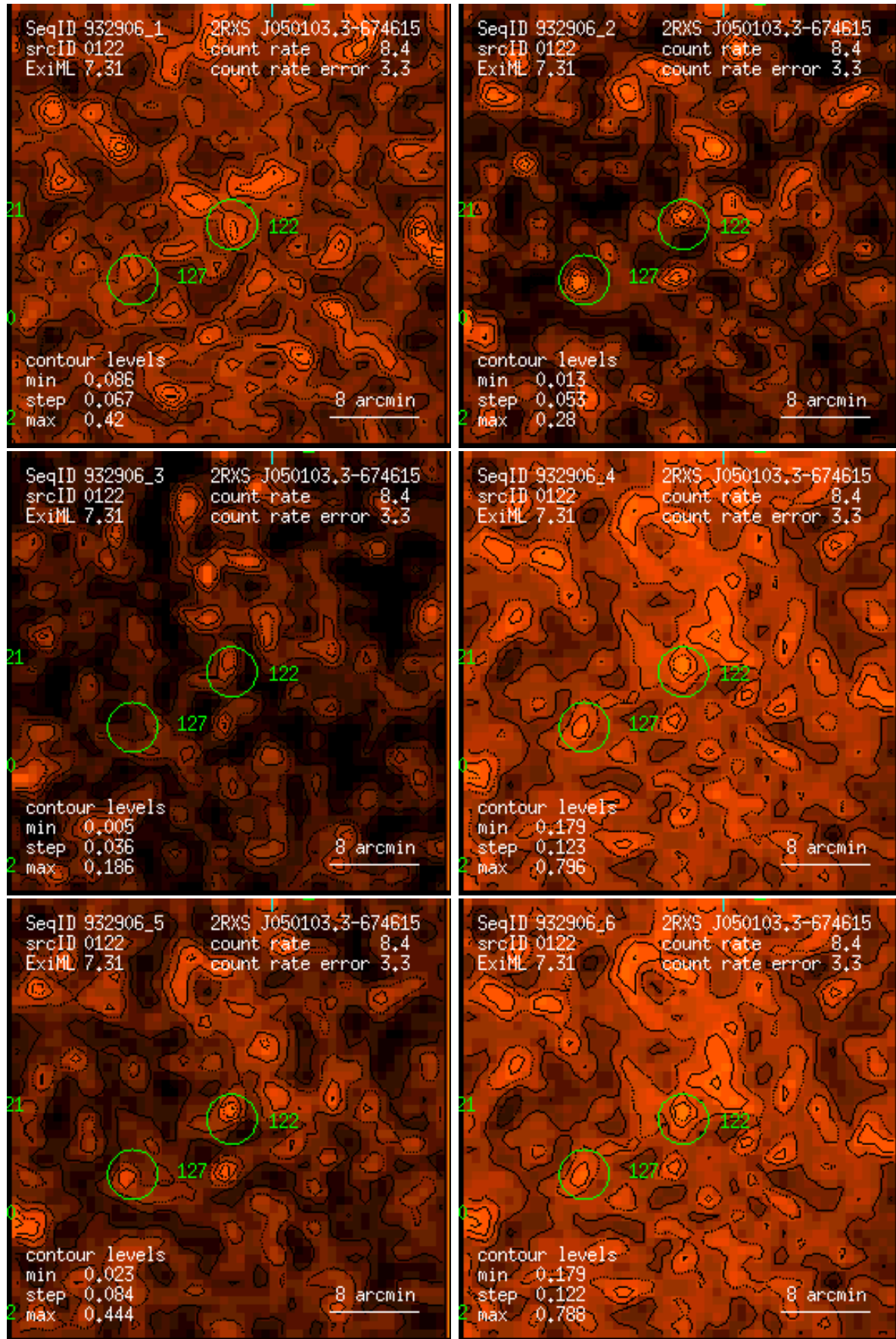
Figure 122: RASS 932906: detection 0122: band rate images, Gaussian filter: (1) PSPC channels 11 – 41, (2) 52 – 90, (3) 91 – 201, (4) 11 – 235, (5) 52 – 201, (6) 11 – 201. Broad band rates in counts/ks. Band rate contour levels in counts/ks/arcmin 2 .
