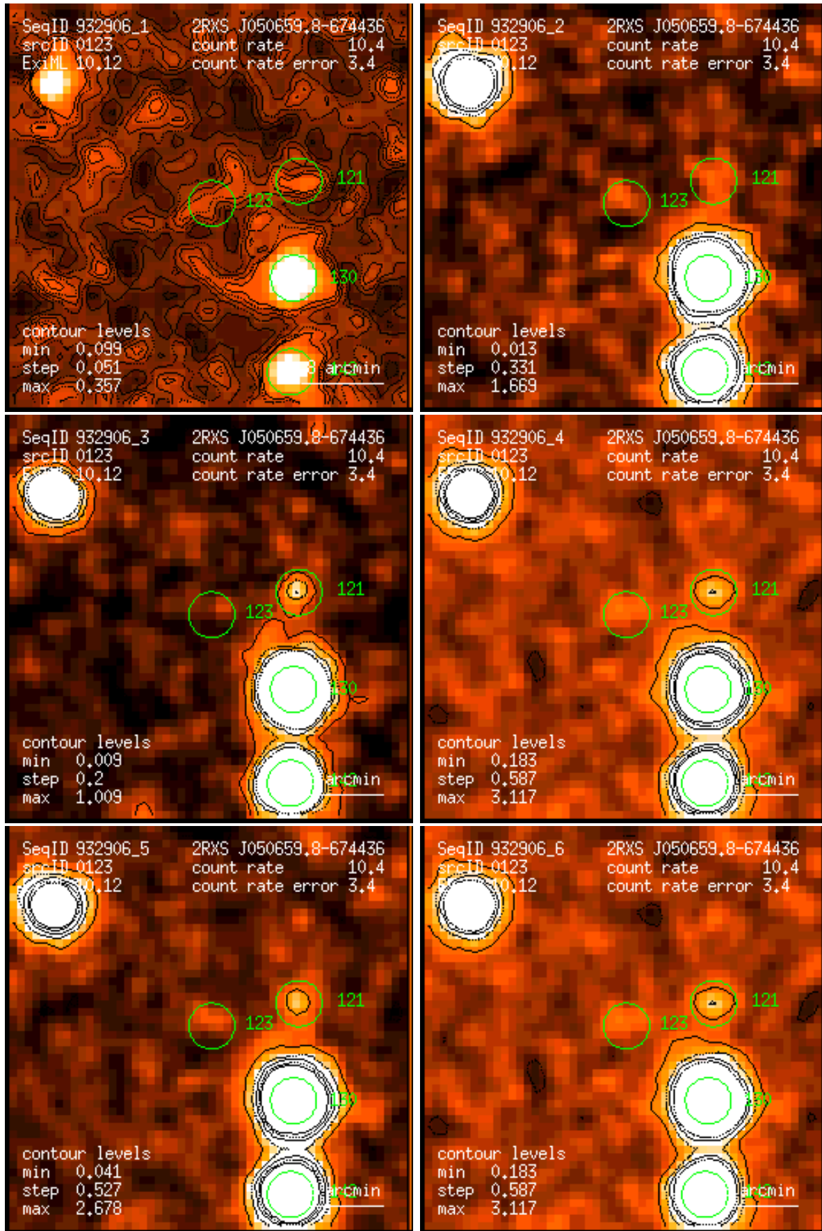
Figure 123: RASS 932906: detection 0123: band rate images, Gaussian filter: (1) PSPC channels 11 – 41, (2) 52 – 90, (3) 91 – 201, (4) 11 – 235, (5) 52 – 201, (6) 11 – 201. Broad band rates in counts/ks. Band rate contour levels in counts/ks/arcmin 2 .
