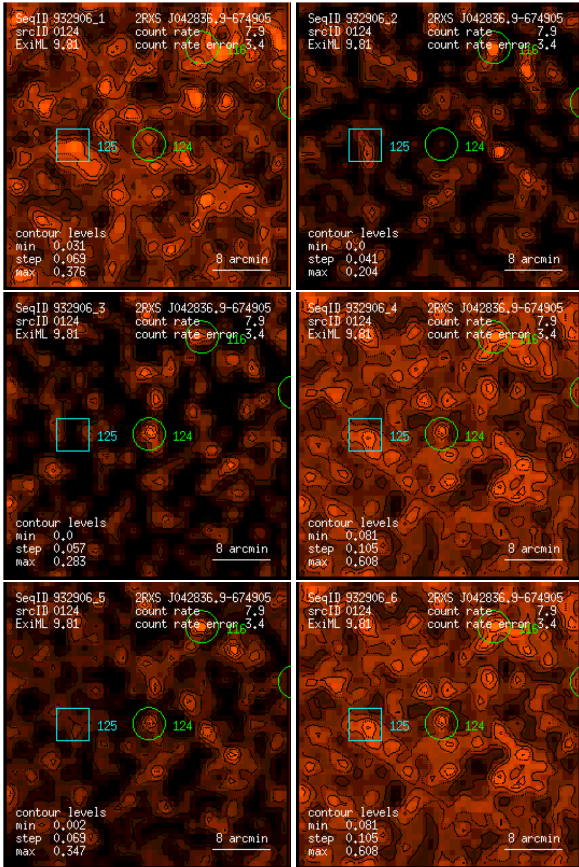
Figure 124: RASS 932906: detection 0124: band rate images, Gaussian filter: (1) PSPC channels 11 – 41, (2) 52 – 90, (3) 91 – 201, (4) 11 – 235, (5) 52 – 201, (6) 11 – 201. Broad band rates in counts/ks. Band rate contour levels in counts/ks/arcmin 2 .
