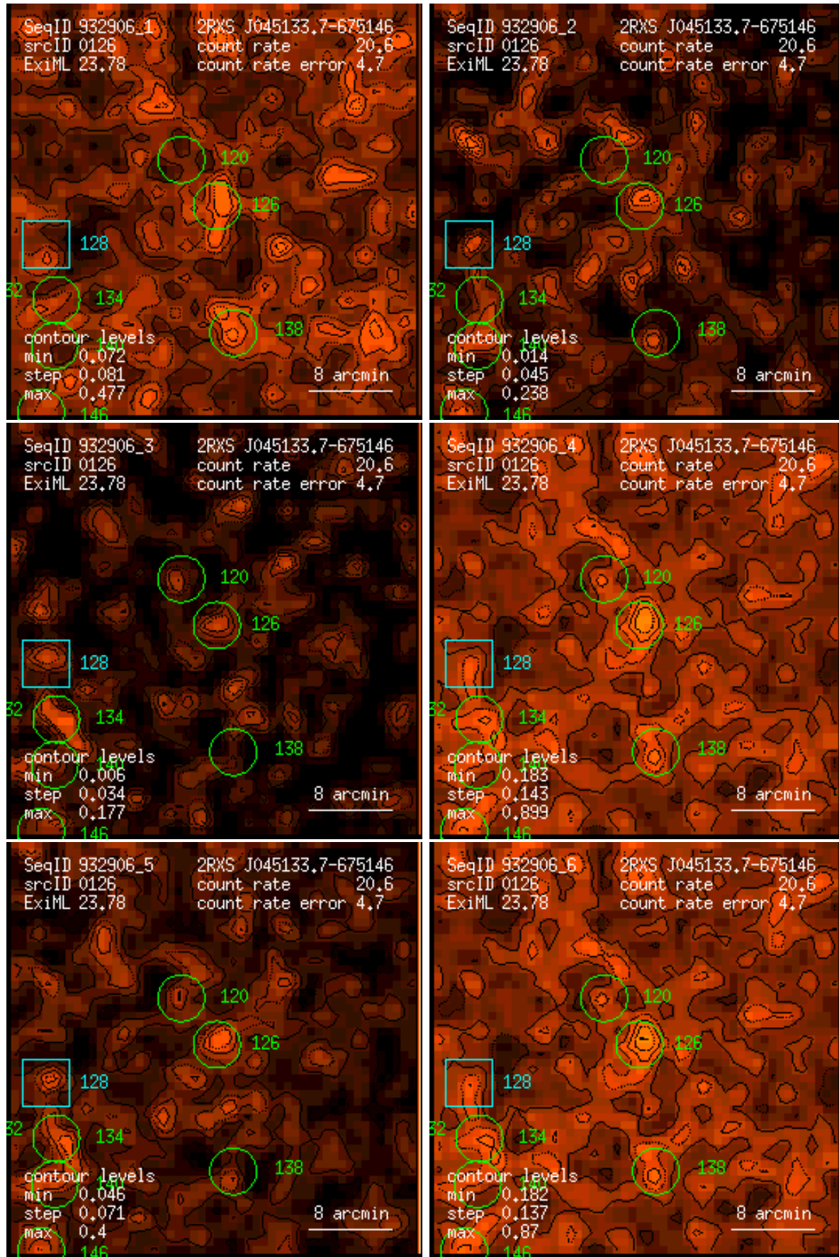
Figure 126: RASS 932906: detection 0126: band rate images, Gaussian filter: (1) PSPC channels 11 – 41, (2) 52 – 90, (3) 91 – 201, (4) 11 – 235, (5) 52 – 201, (6) 11 – 201. Broad band rates in counts/ks. Band rate contour levels in counts/ks/arcmin 2 .
