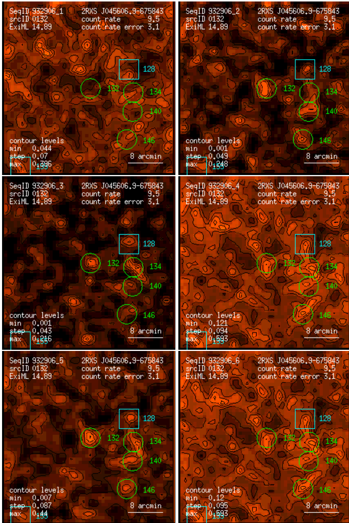
Figure 132: RASS 932906: detection 0132: band rate images, Gaussian filter: (1) PSPC channels 11 – 41, (2) 52 – 90, (3) 91 – 201, (4) 11 – 235, (5) 52 – 201, (6) 11 – 201. Broad band rates in counts/ks. Band rate contour levels in counts/ks/arcmin 2 .
