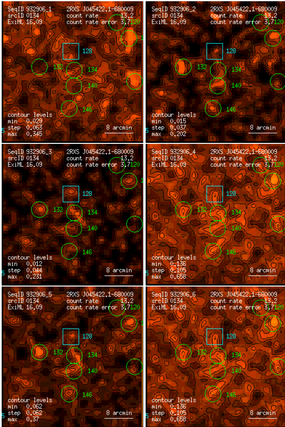
Figure 134: RASS 932906: detection 0134: band rate images, Gaussian filter: (1) PSPC channels 11 – 41, (2) 52 – 90, (3) 91 – 201, (4) 11 – 235, (5) 52 – 201, (6) 11 – 201. Broad band rates in counts/ks. Band rate contour levels in counts/ks/arcmin 2 .
