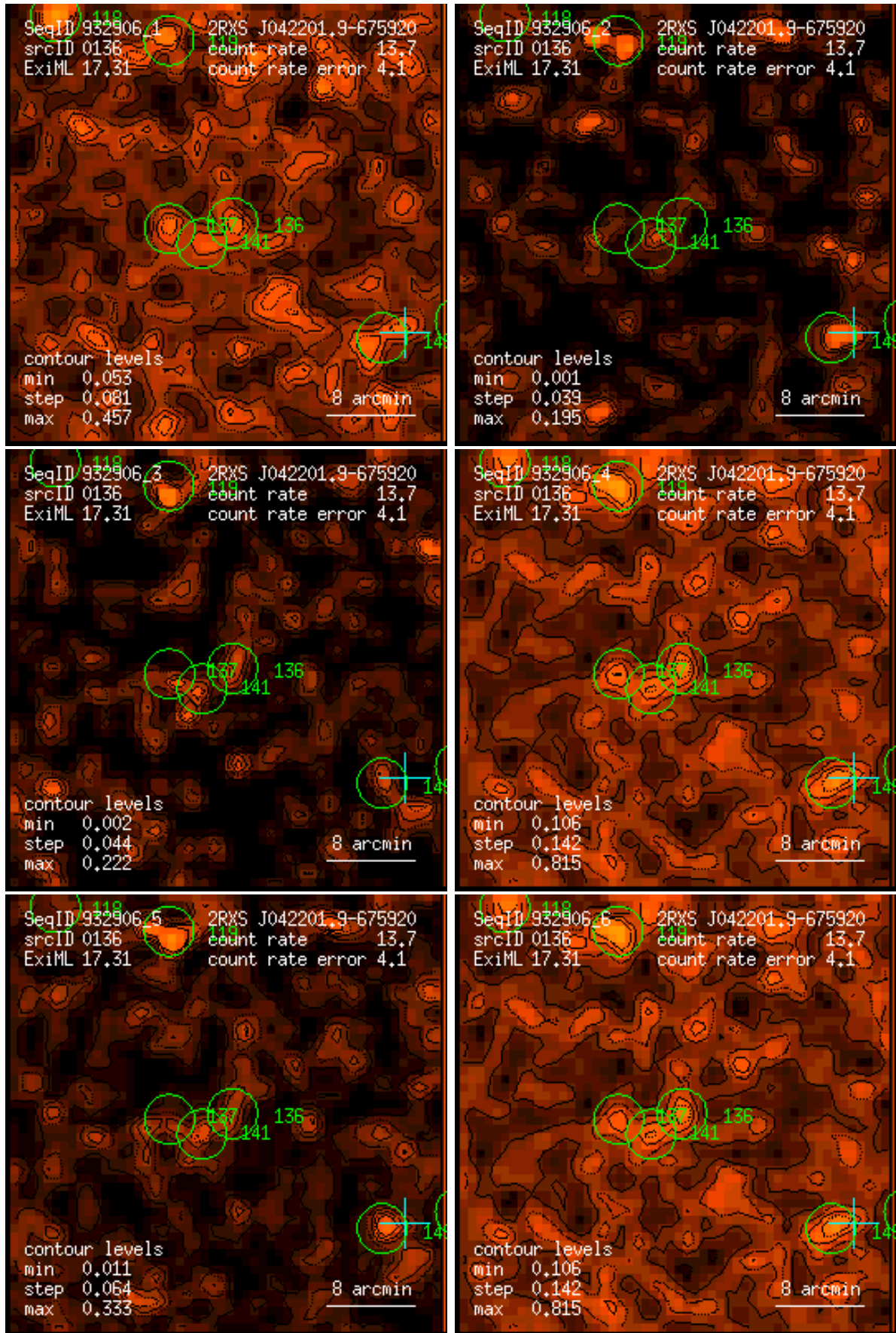
Figure 136: RASS 932906: detection 0136: band rate images, Gaussian filter: (1) PSPC channels 11 – 41, (2) 52 – 90, (3) 91 – 201, (4) 11 – 235, (5) 52 – 201, (6) 11 – 201. Broad band rates in counts/ks. Band rate contour levels in counts/ks/arcmin 2 .
